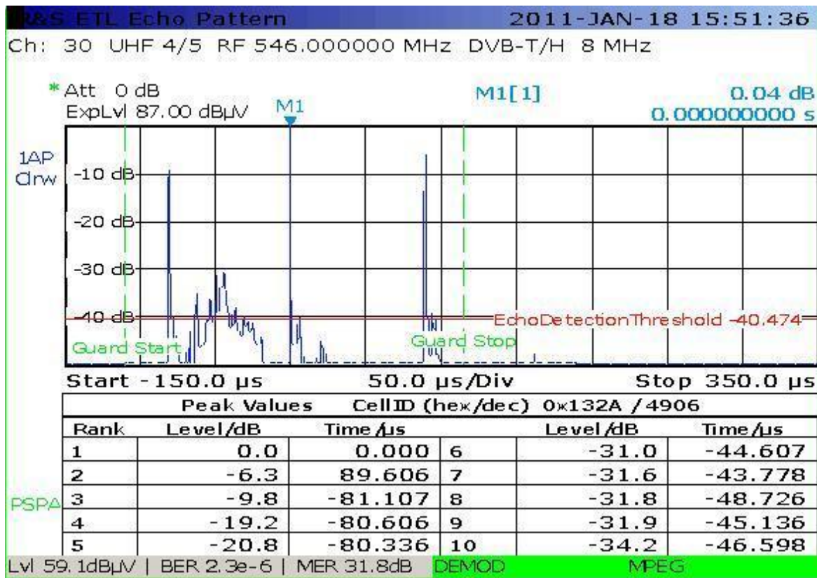
FIGURE 9 Impulse response for MUX2 at Gravedona measurement point
