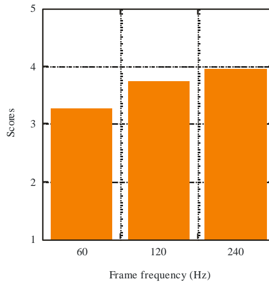
FIGURE 18 Average score
