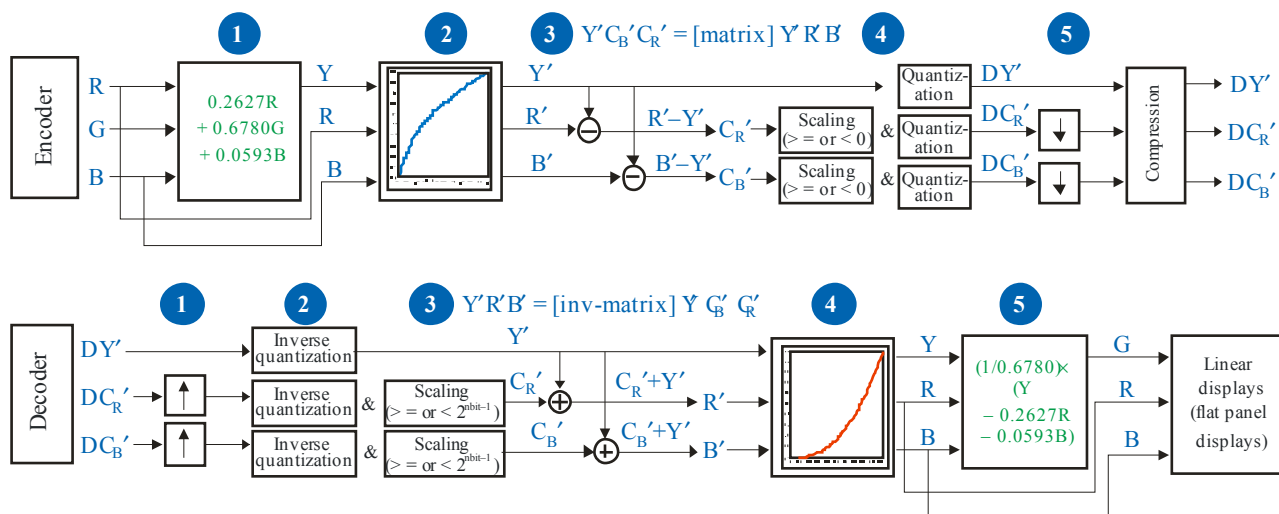
The CL colour encoding method
