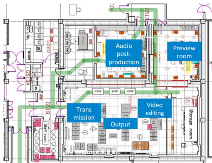
BBC TCO studio layout
