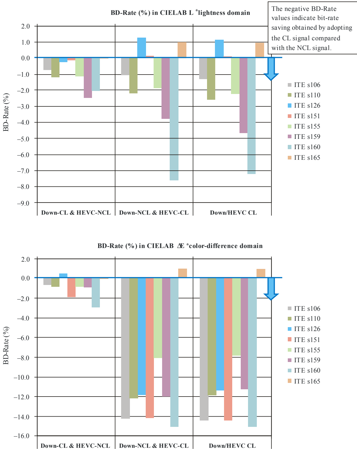
(a) The BD-Rate (%) in the CIELAB lightness and colour-difference domains (The estimated bit-rate saving by applying the CL for either down-sampling or compression in replacement of the NCL)
