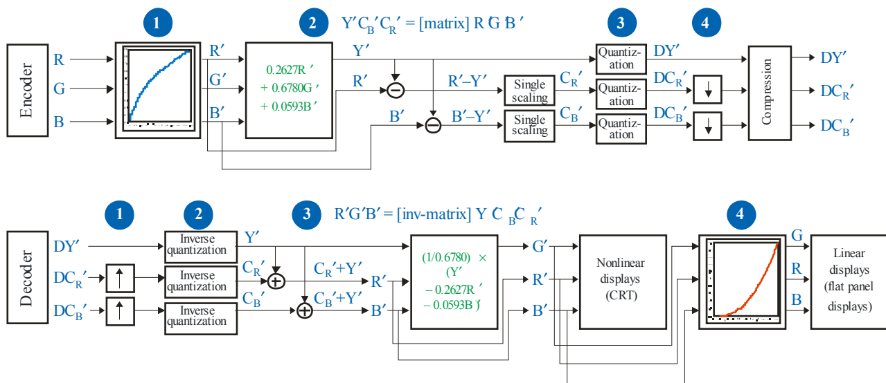
The NCL colour encoding method
