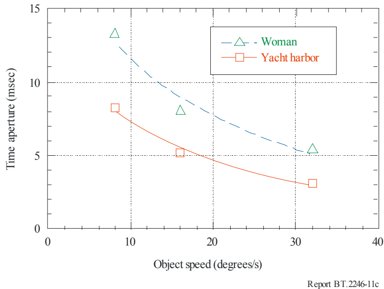
FIGURE 12c Relationship between time aperture and object speed giving an acceptable level of motion blur
