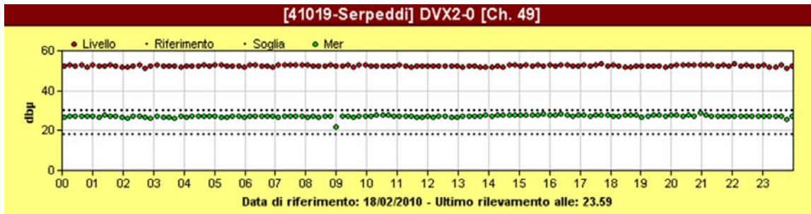
MER chart (threshold values are defined by ETSI)
