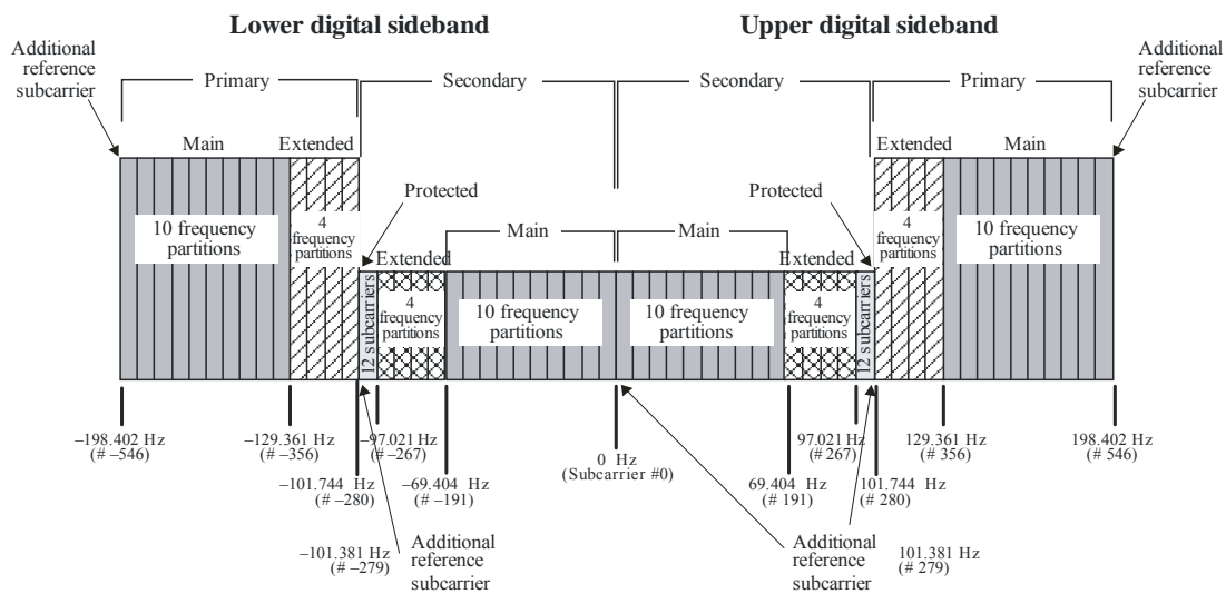
Spectrum of the all-digital waveform (The level of the digital subcarriers is such that the total power of these carriers is no more than 10 dB below the nominal power of the FM analogue carrier that it replaces)
