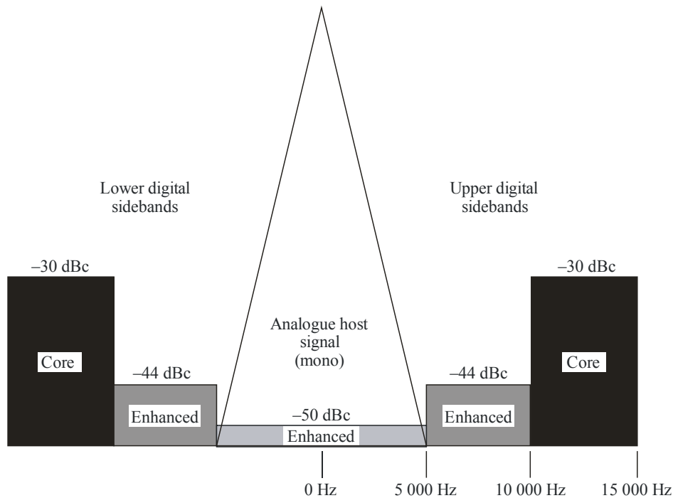
FIGURE 7 Hybrid MF IBOC DSB power spectral density
