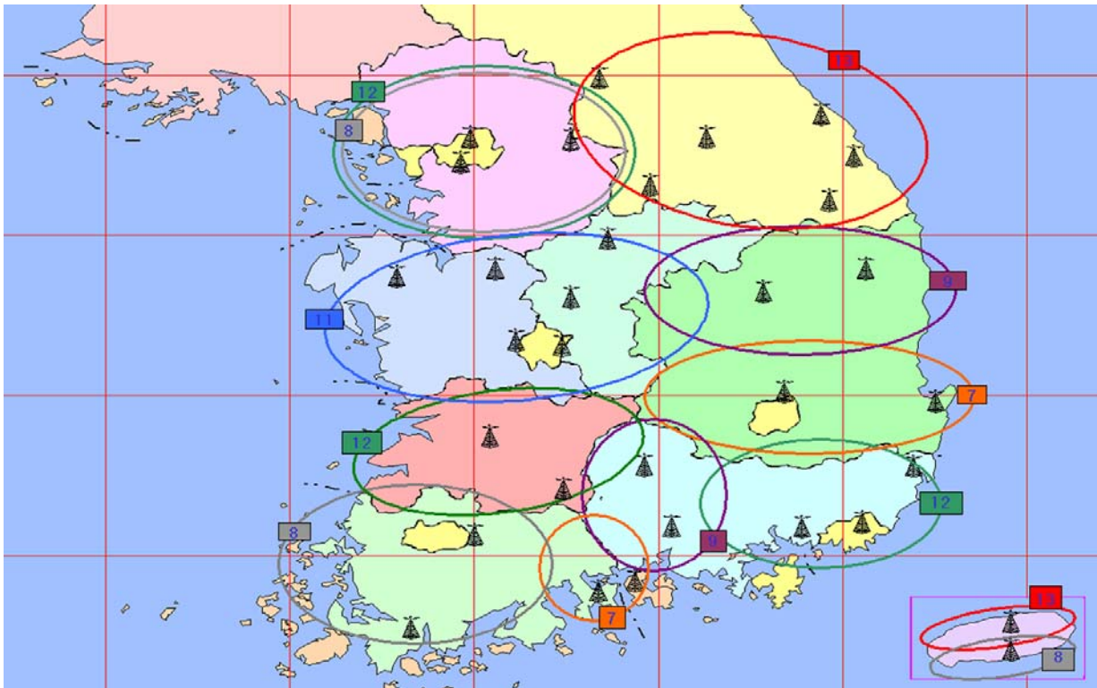
FIGURE 57 Channel Assignments for T-DMB in Korea
