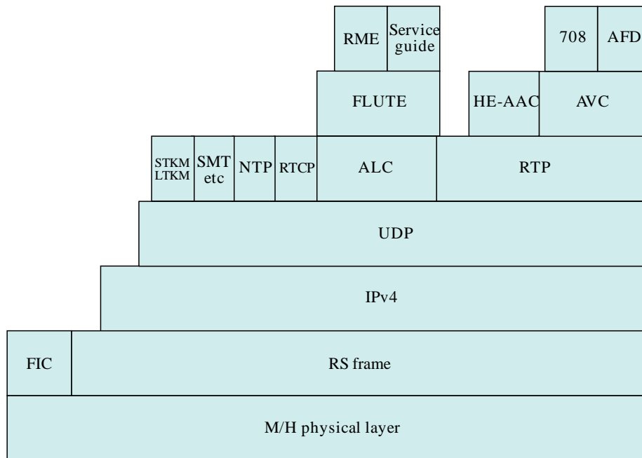
FIGURE 23 ATSC-M/H broadcast protocol stack
