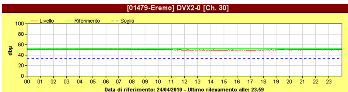
FIGURE 46 RF Charts
