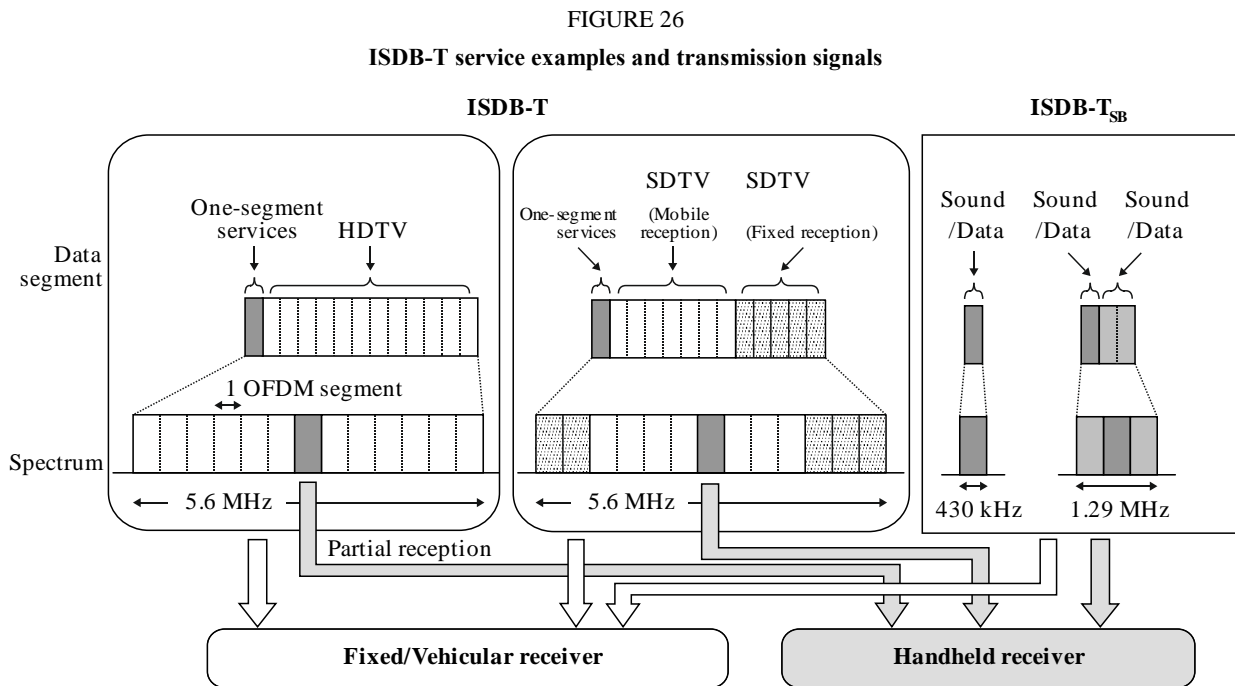
ISDB-T service examples and transmission signals
