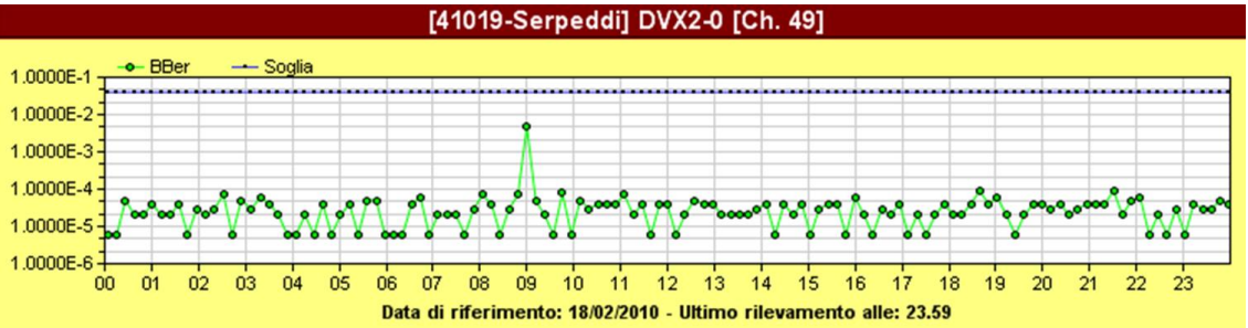
FIGURE 48 BER chart
