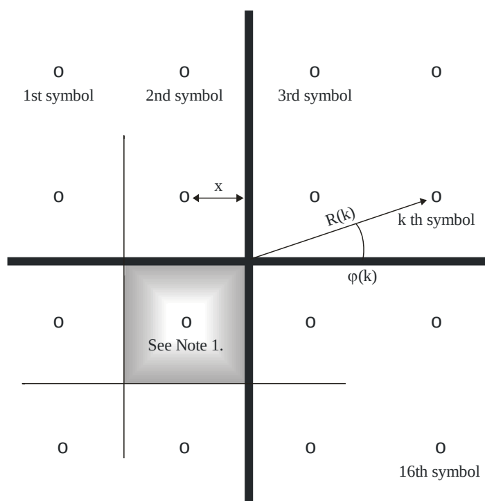
FIGURE 3 Constellation 16-QAM
