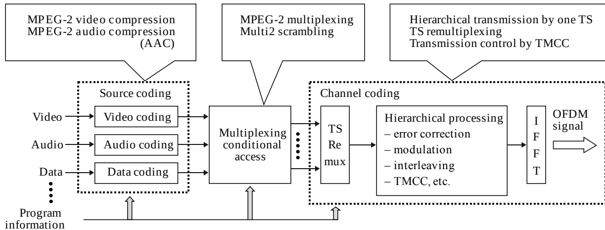
ISDB-T system configuration
