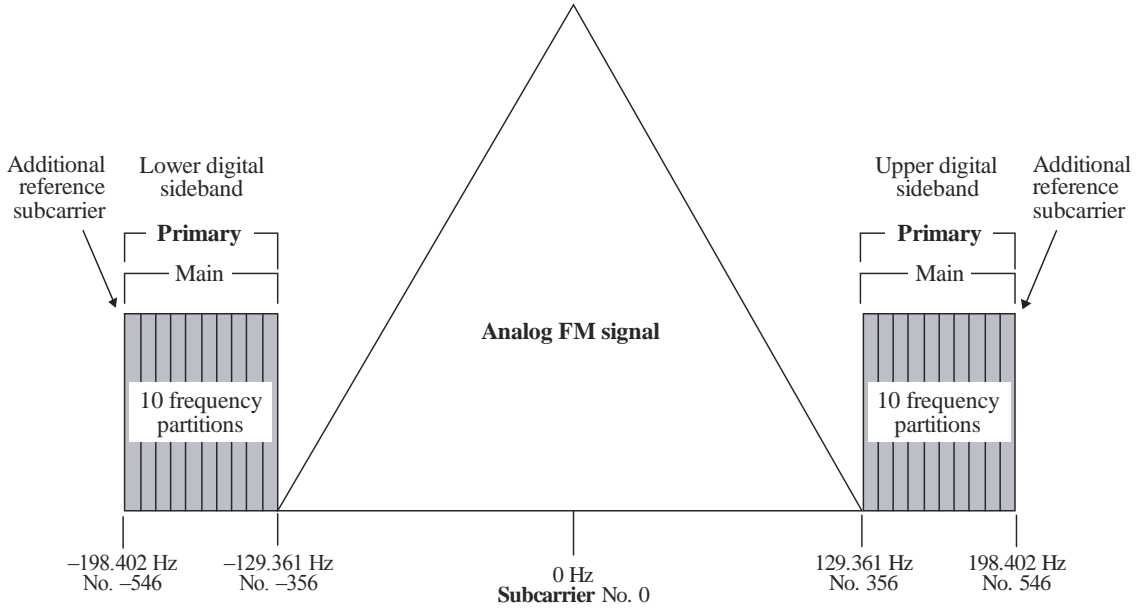
Spectrum of the hybrid waveform—service mode (The level of the digital subcarriers is such that the total power of these carriers is 20 dB below the nominal power of the FM analogue carrier)
