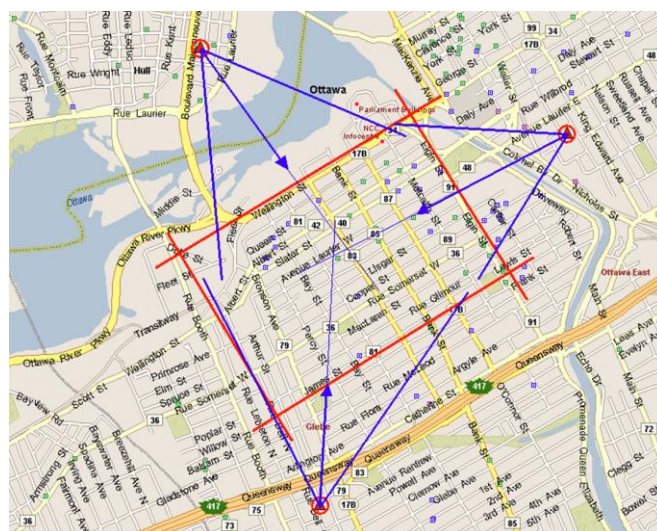
Ottawa distributed translator network. The rectangular target area is 1.6 × 1.14 km
