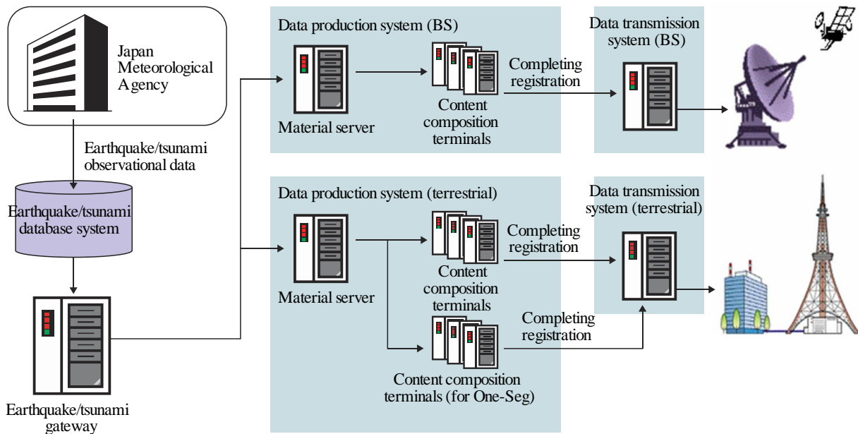
System configuration and flow for earthquake and tsunami information
