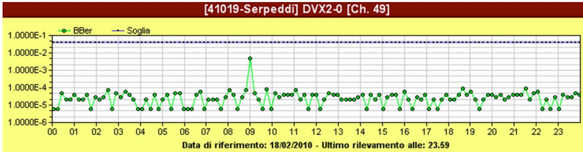
FIGURE 48 BER chart
