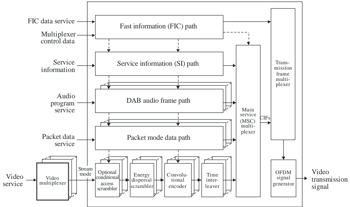
FIGURE 29 Conceptual transmission architecture for the video services DAB (ETSI EN 300 401)
