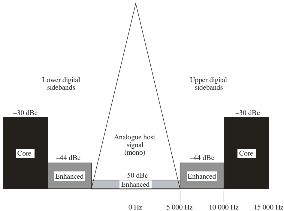
FIGURE 9 Hybrid MF IBOC DSB power spectral density
