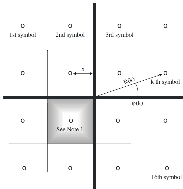
FIGURE 3 Constellation 16-QAM
