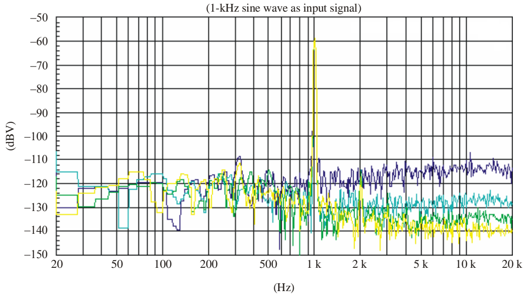
FIGURE 15 Audio frequency response of analogue radio microphone
