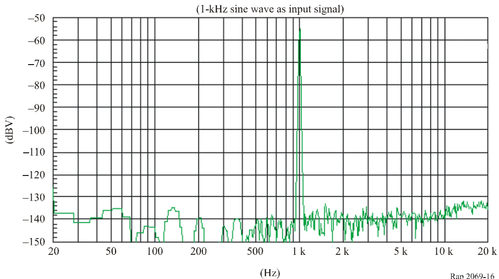
FIGURE 16 Audio frequency response of digital radio microphone
