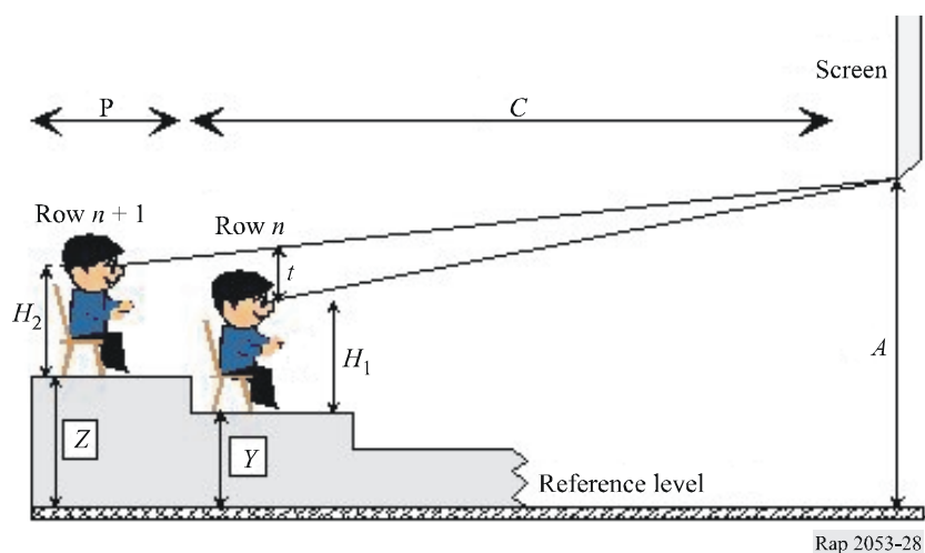
FIGURE 28 Head clearance
