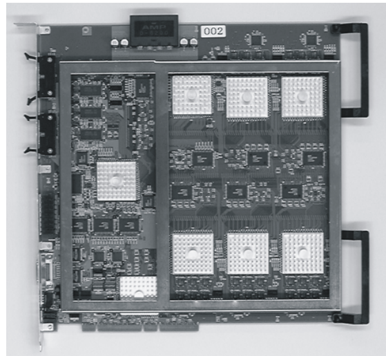
FIGURE 20 JPEG2000 decoder board
