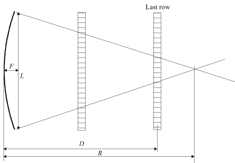
FIGURE 24 Screen curvature radius
