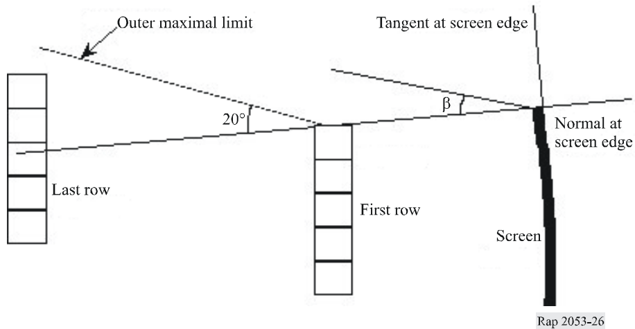
FIGURE 26 Side vision angle, curved screen
