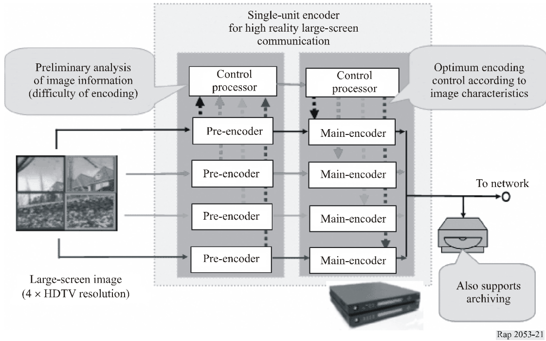
FIGURE 21 Spatially parallel encoding architecture for LSDI
