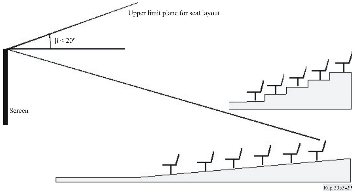
FIGURE 29 Seat upper limit plane
