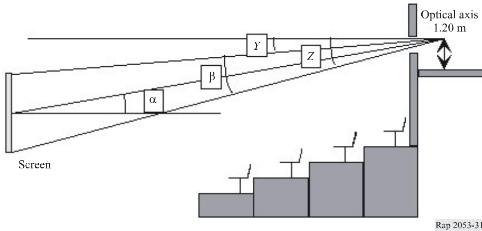
FIGURE 31 Image geometric distortion (vertical)
