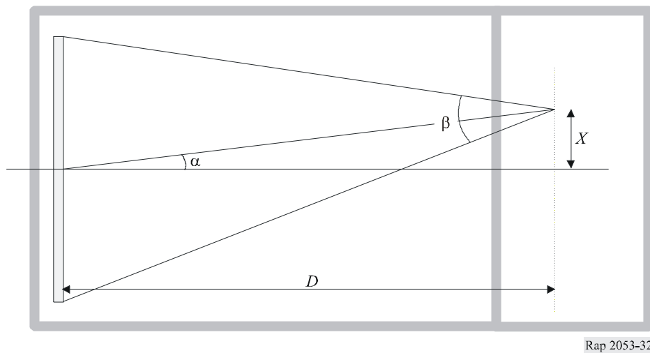
FIGURE 32 Image geometric distortion (horizontal)
