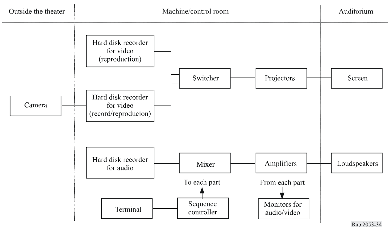
FIGURE 34 Schematic diagram
