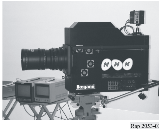
FIGURE 3 External view of experimental camera
