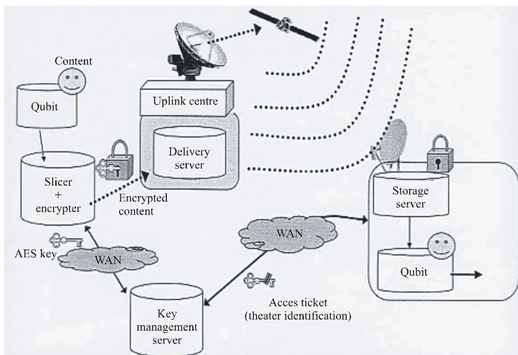
FIGURE 38 Distribution network for LSDI content
