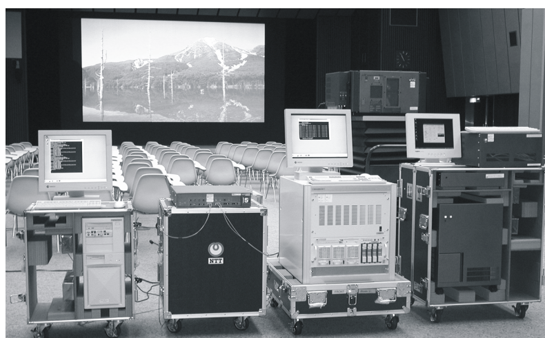
FIGURE 19 Overview of prototype SHD movie system
