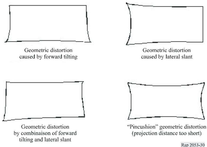
FIGURE 30 Image geometric distortion
