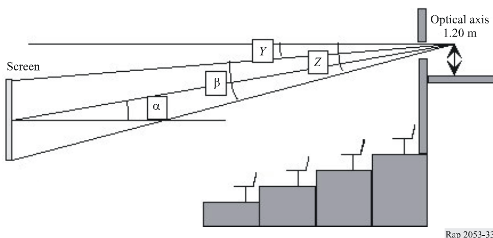
FIGURE 33 Clearance under projection beam
