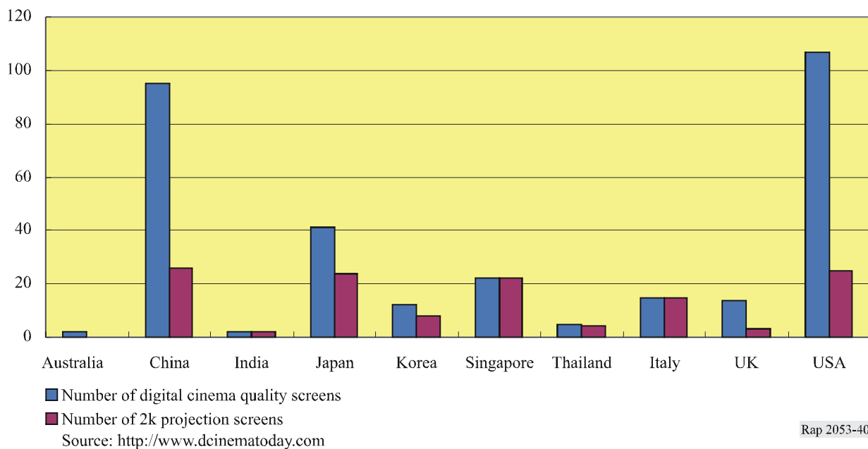
FIGURE 40 Number of LSDI screens
