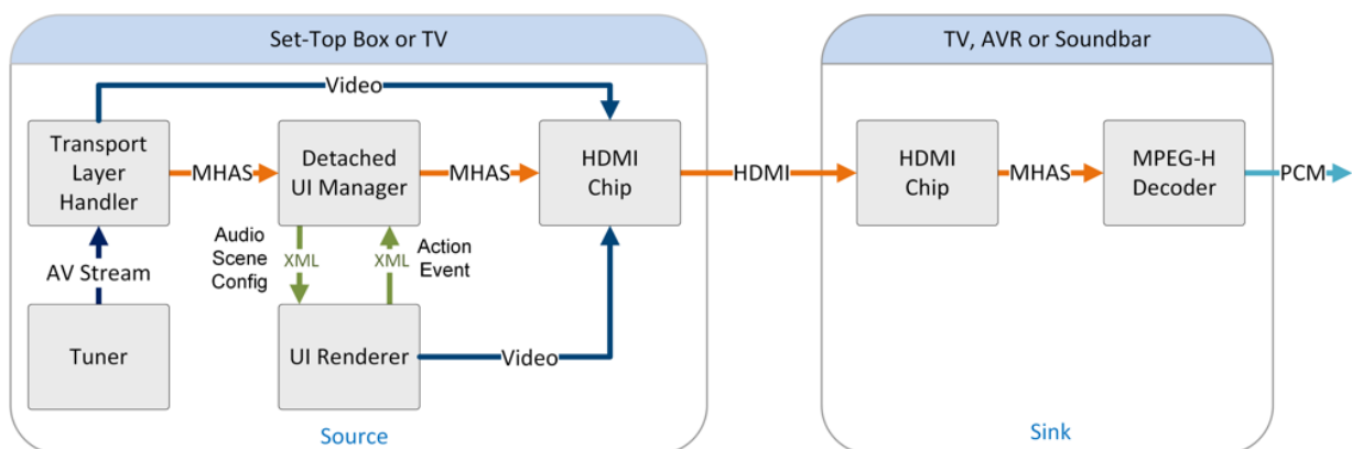
Distributed UI processing with transmission of user commands over HDMI
