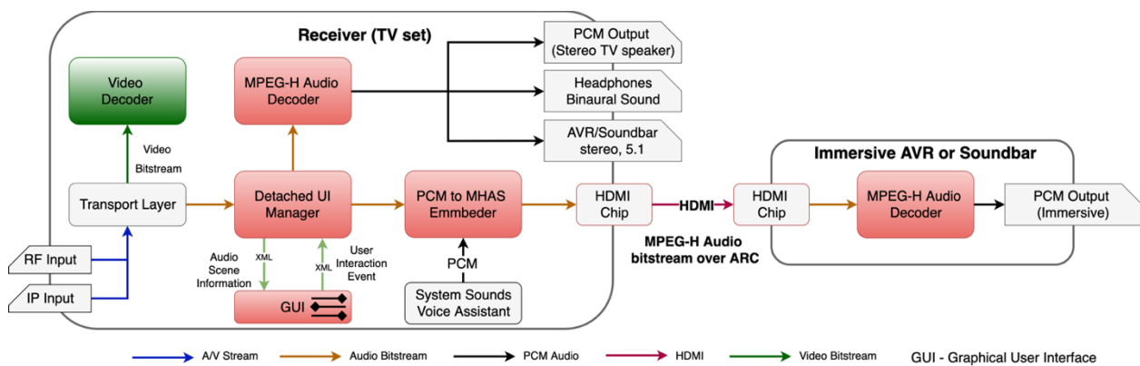
Top level block diagram of a receiver using MPEG-H Audio
