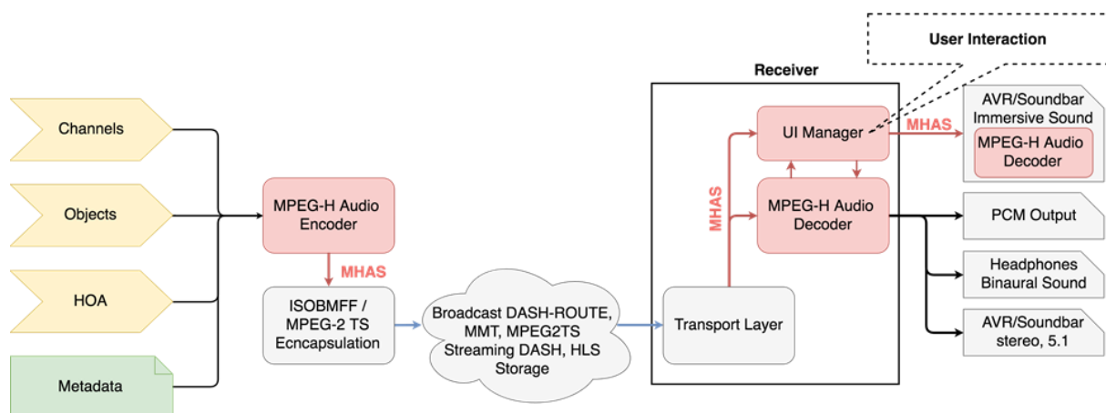
FIGURE 15 Overview of the MPEG-H Audio System
