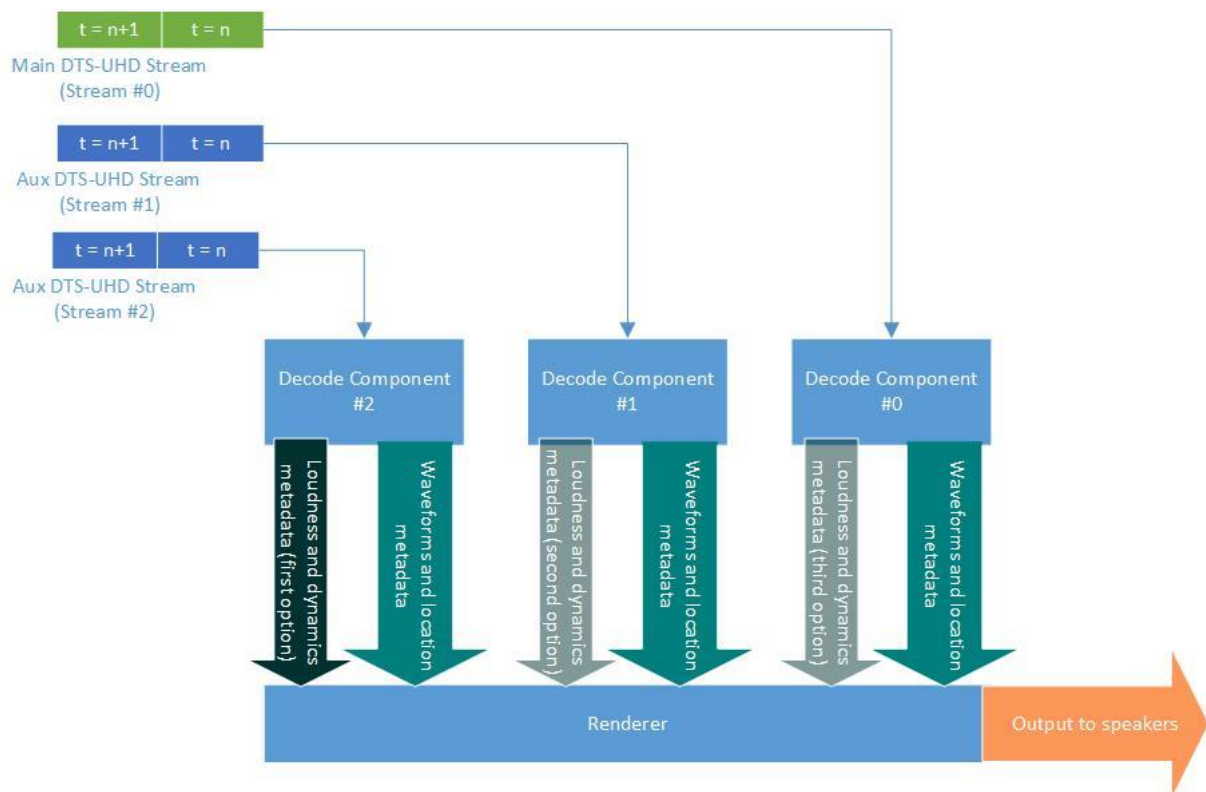
FIGURE 36 Multi-stream support
