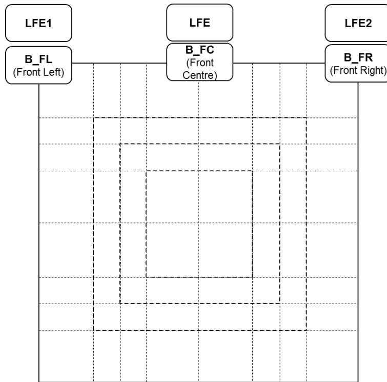
d) Typical loudspeaker labels for general layers
