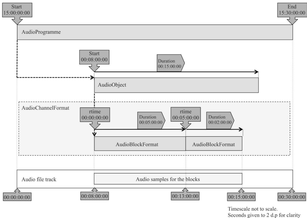
FIGURE 2 Timing diagram
