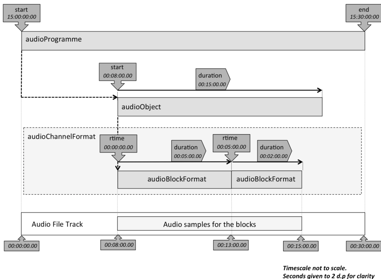
FIGURE 1 Timing diagram
