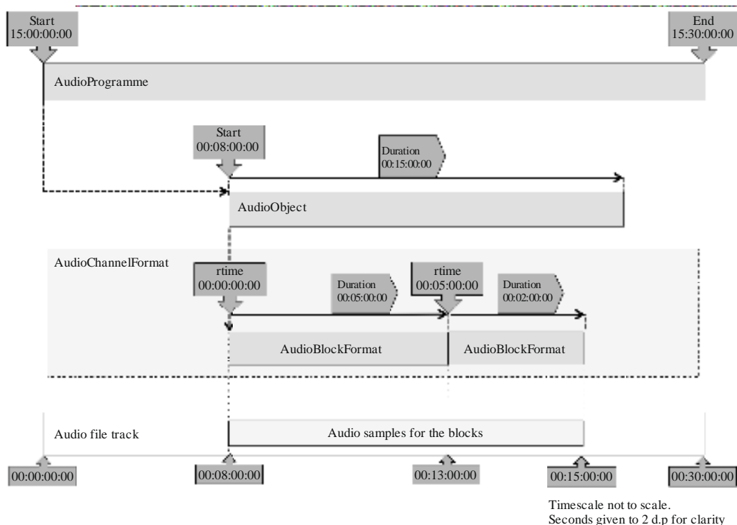
FIGURE 1 Timing diagram
