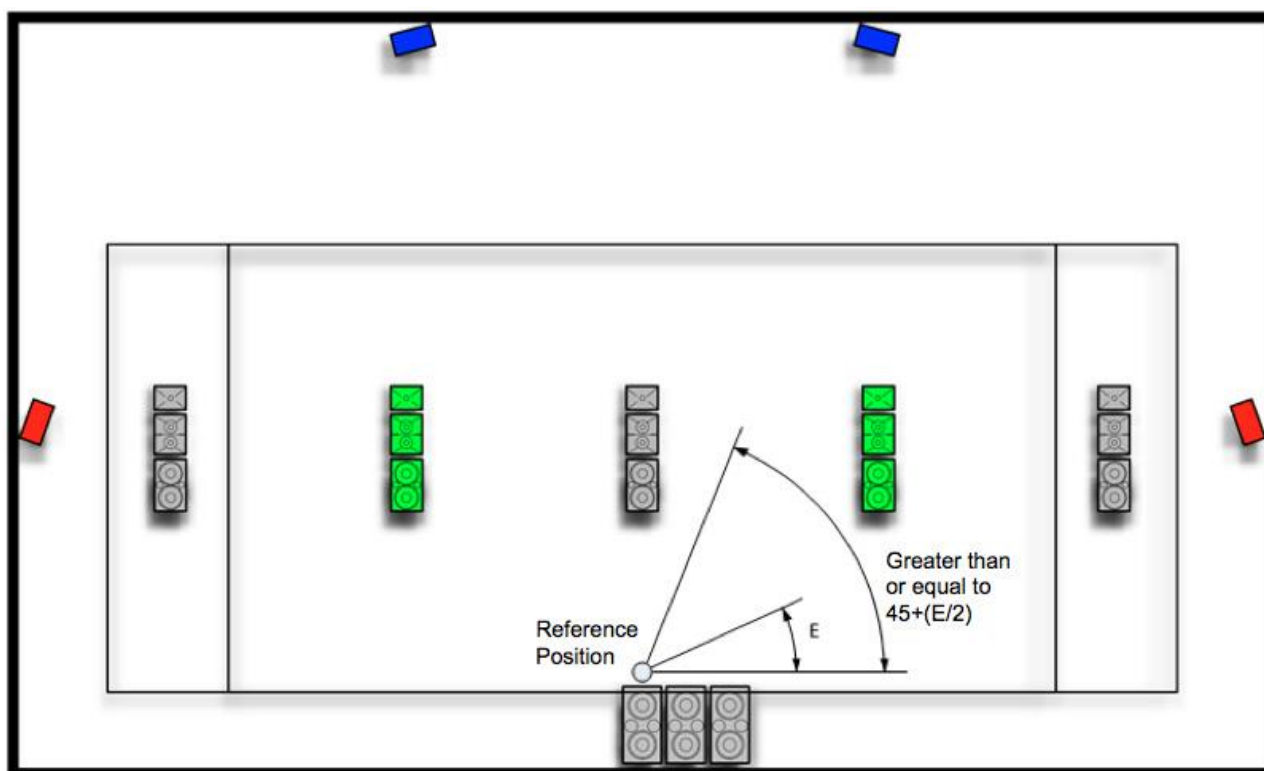
FIGURE 23 Example of top surround lateral position
