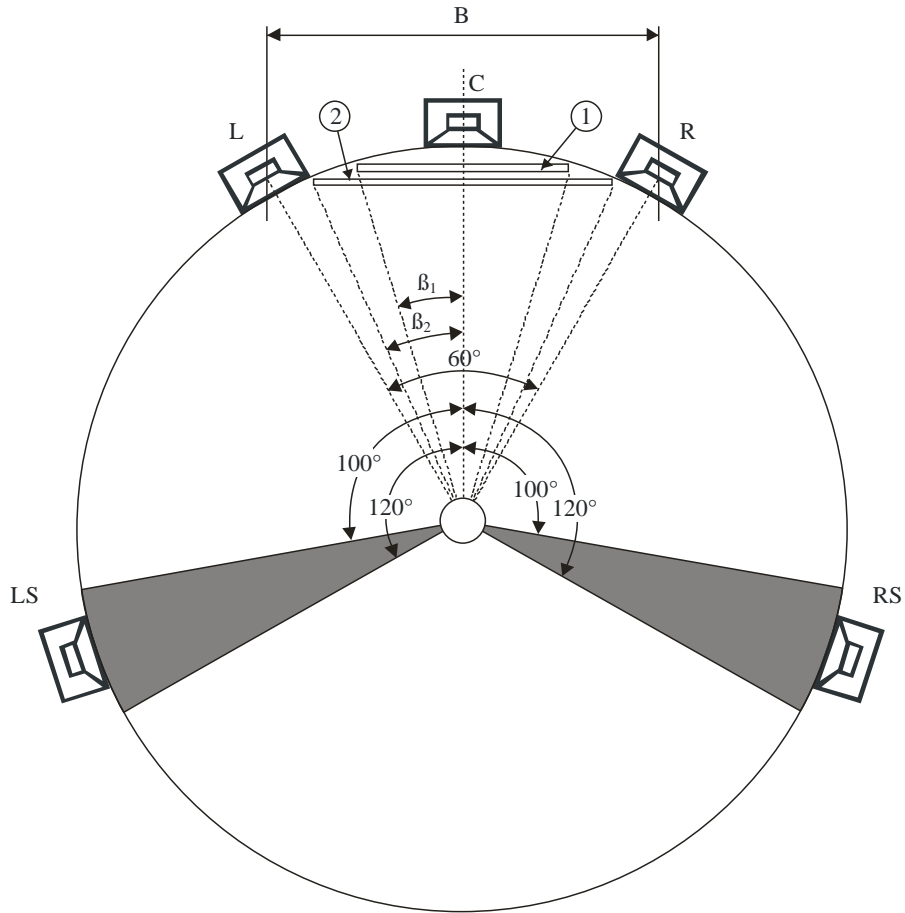
Reference loudspeaker arrangement with loudspeakers L/C/R an LS/RS
