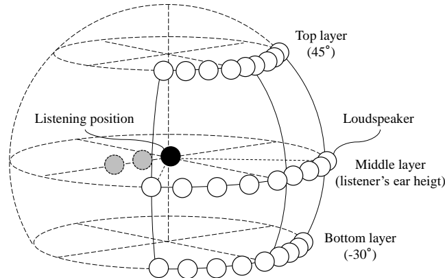
FIGURE 60 Loudspeaker layout in frontal hemispherical plane
