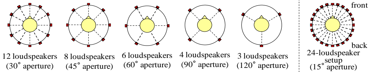
FIGURE 55 Loudspeaker configurations for subjective test and 24-loudspeaker setup
