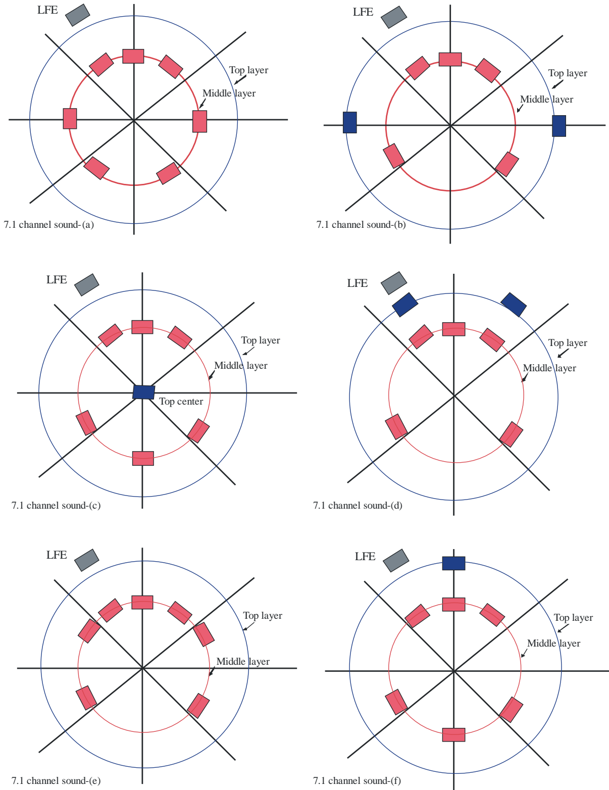
FIGURE 24 Examples of loudspeaker mapping of 7.1 channel sound
