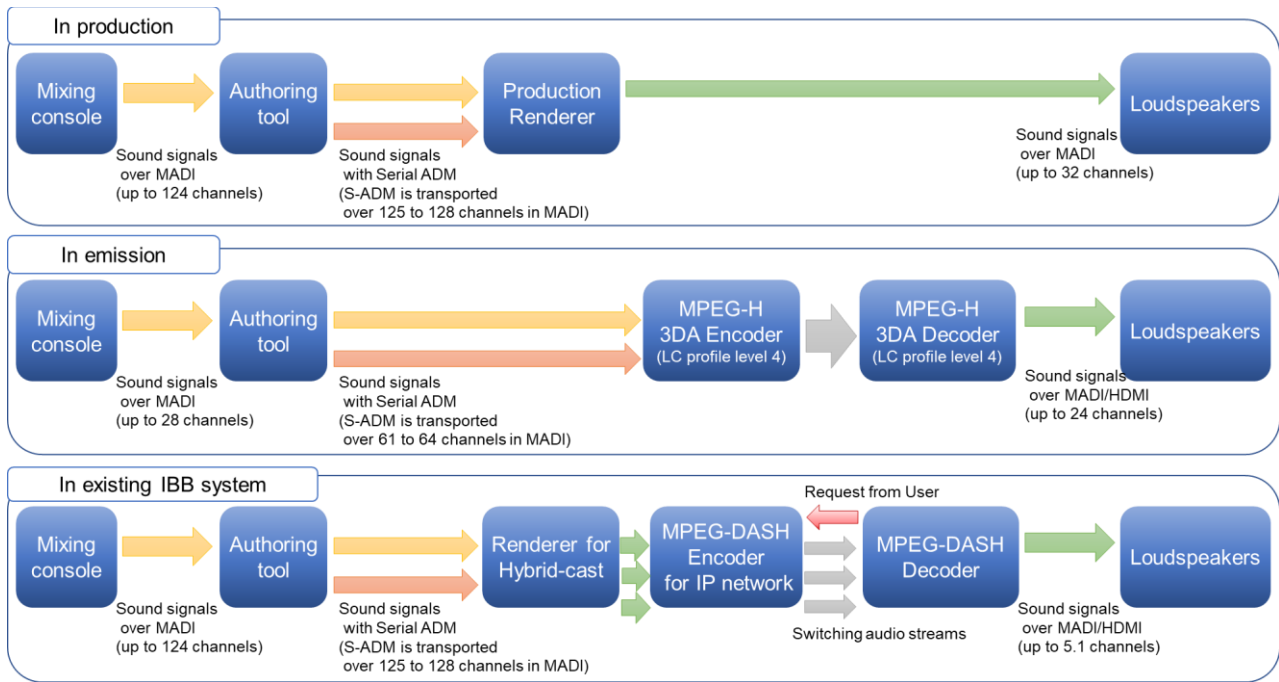
FIGURE 32 Application of Serial ADM (S-ADM)
