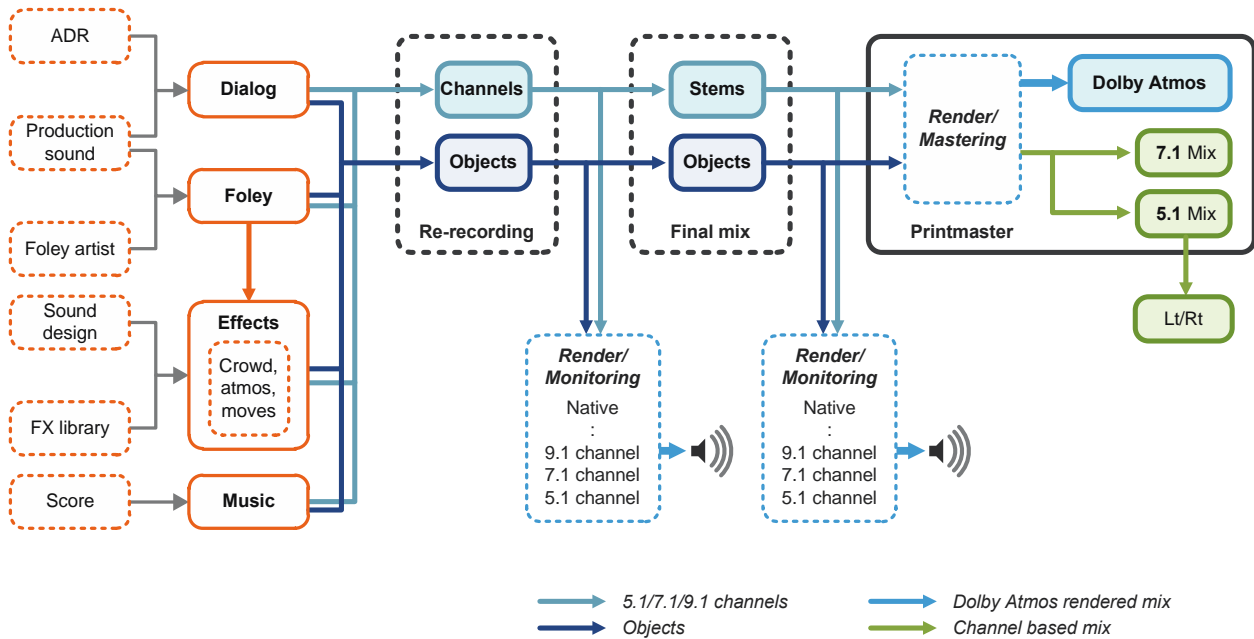
Authoring workflow, showing combination of channels and objects
