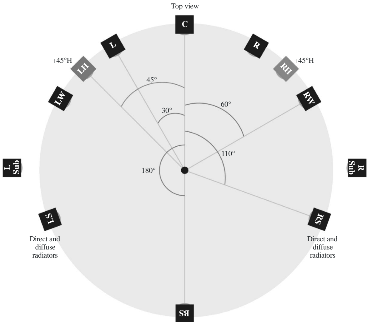
FIGURE 7 Diagram of speaker layout for 10.2
