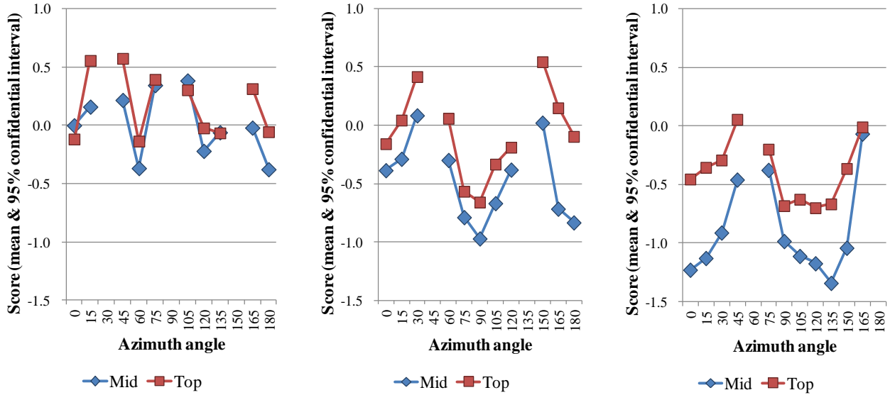
(a) 6 loudspeakers
