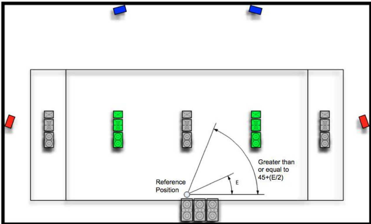
FIGURE 23 Example of top surround lateral position
