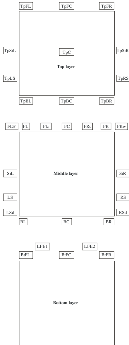
FIGURE 60 Layers and channel assignment
