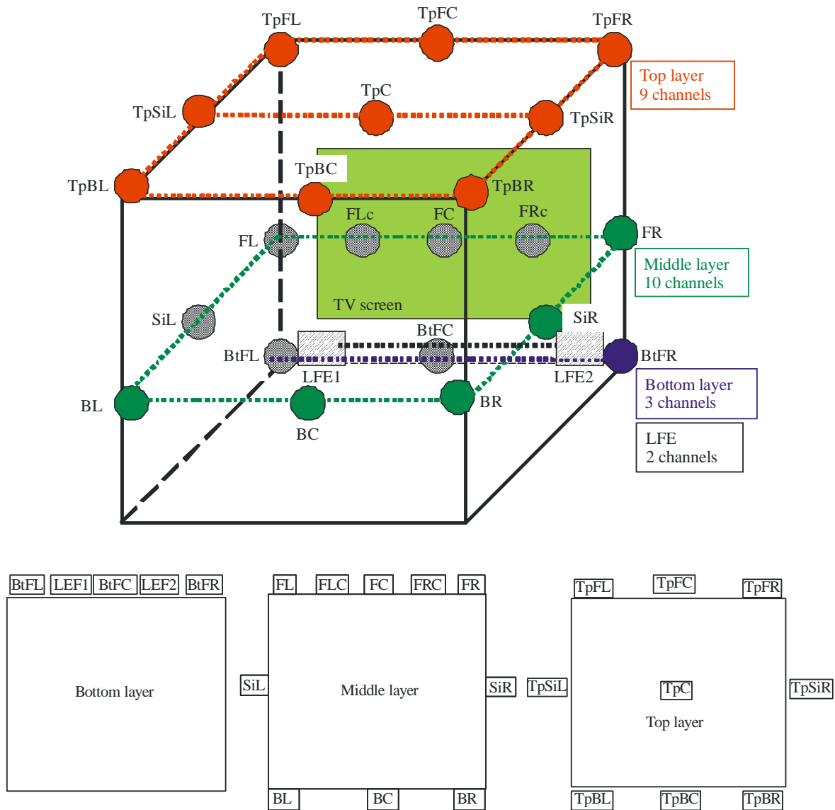
FIGURE 2 The 22.2 multichannel sound system
