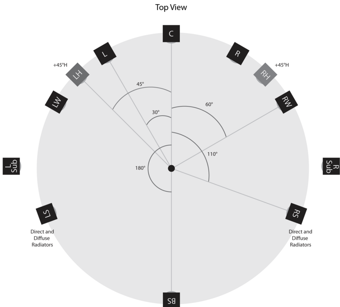
FIGURE 7 Diagram of speaker layout for 10.2
