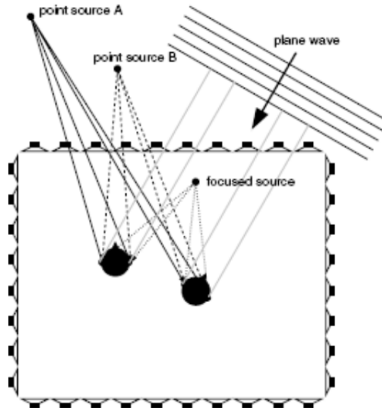
FIGURE 11 Reproduction of point sources, focused sources and plane waves
