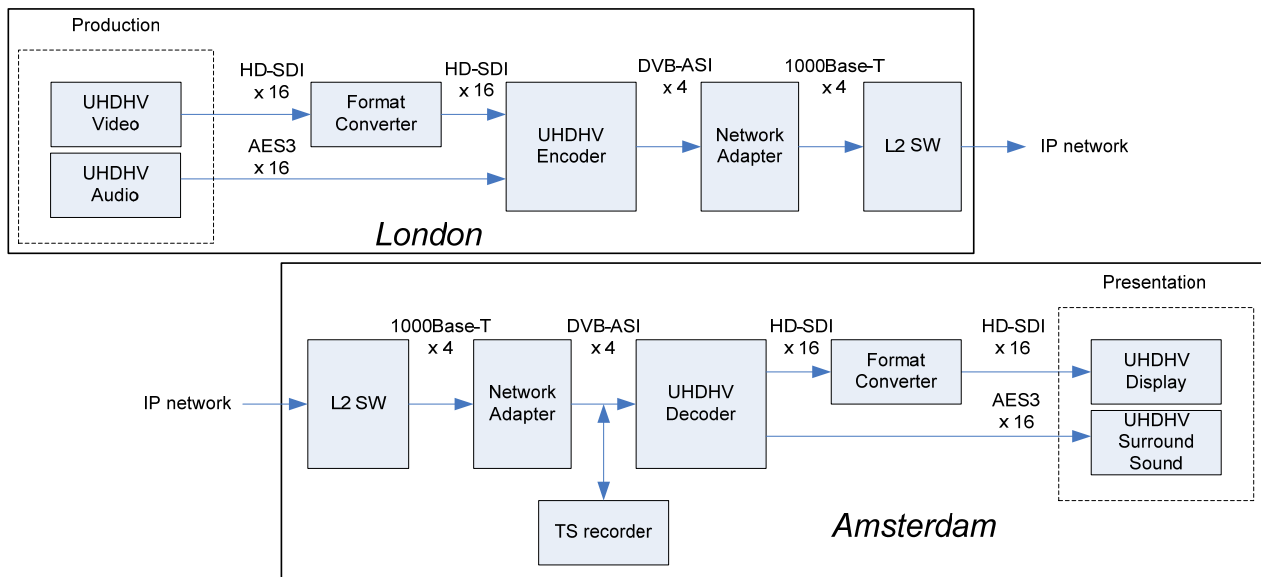
FIGURE 15 UHDTV and 22.2 multichannel sound IP transmission system at IBC2008
