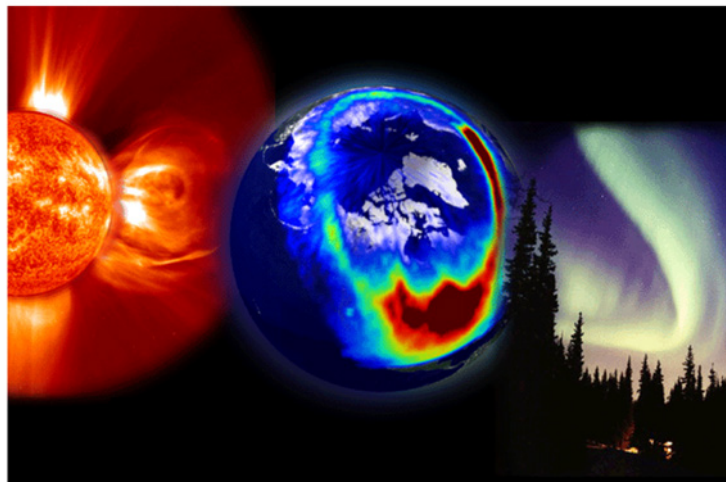
FIGURE 3: Solar activity seen from a satellite and from the ground
