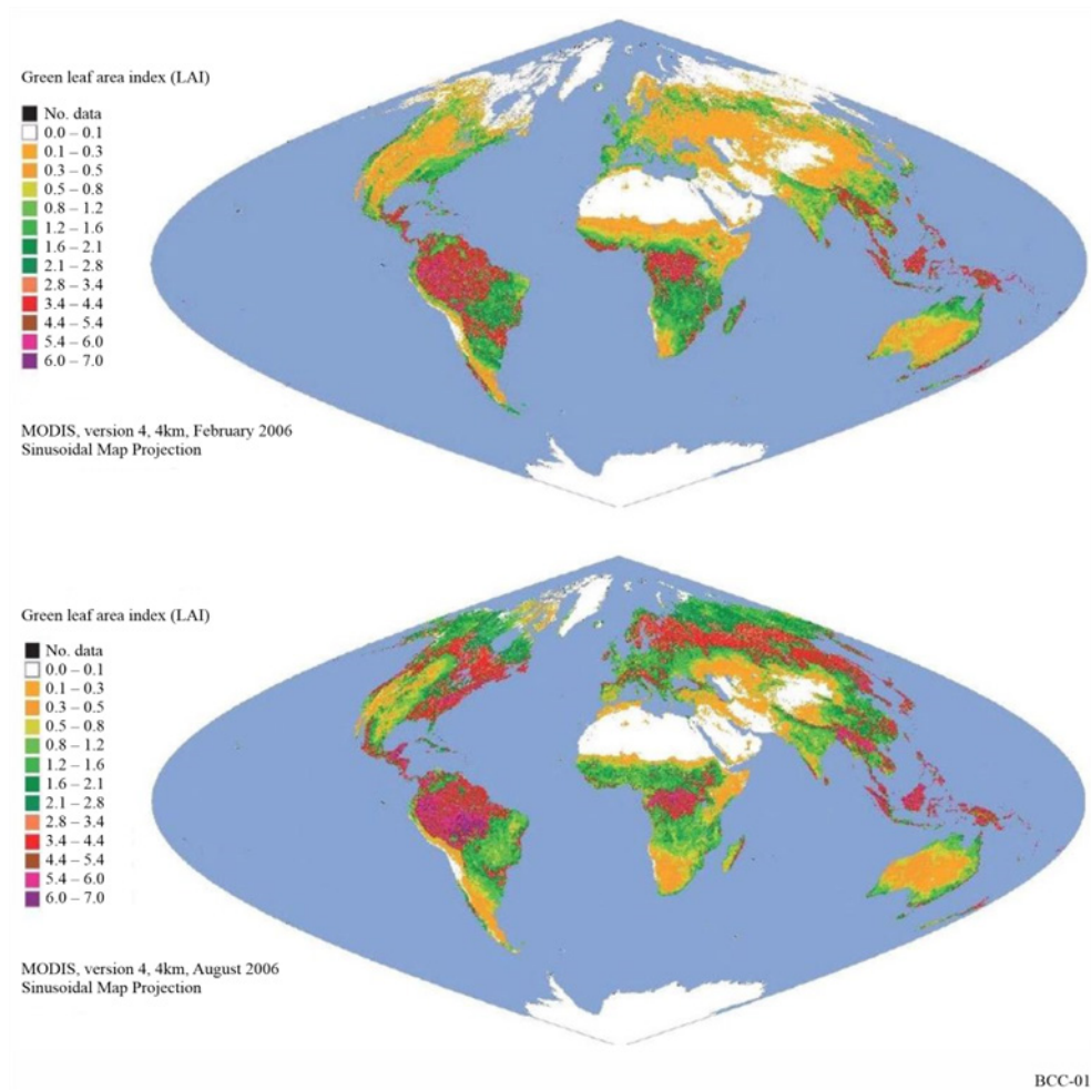
FIGURE 1 : Green Leaf Indices from MODIS showing seasonal changes in vegetation
