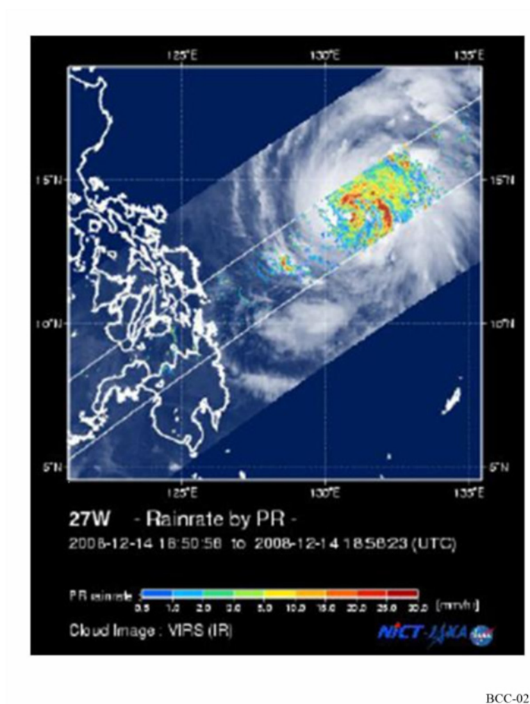
FIGURE 2: Rain rate distribution of a typhoon
