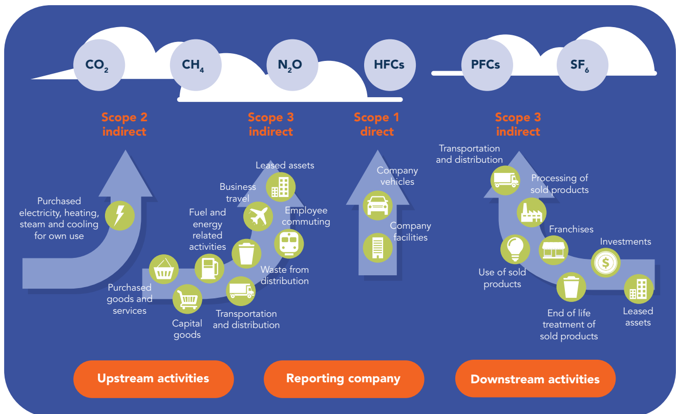
Figure 1.1: Emissions scopes
