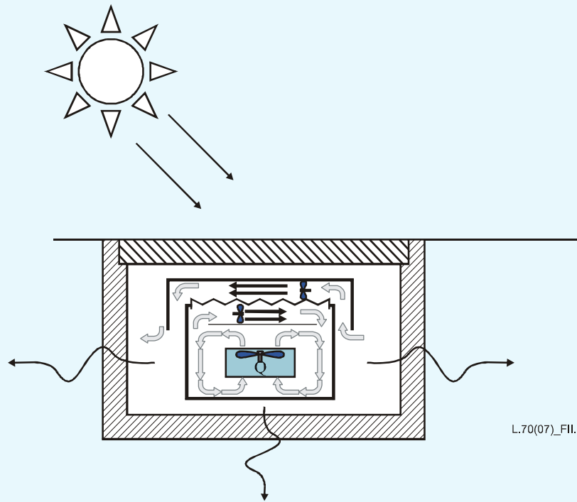
Figure 4A3-2: Heat exchanger
