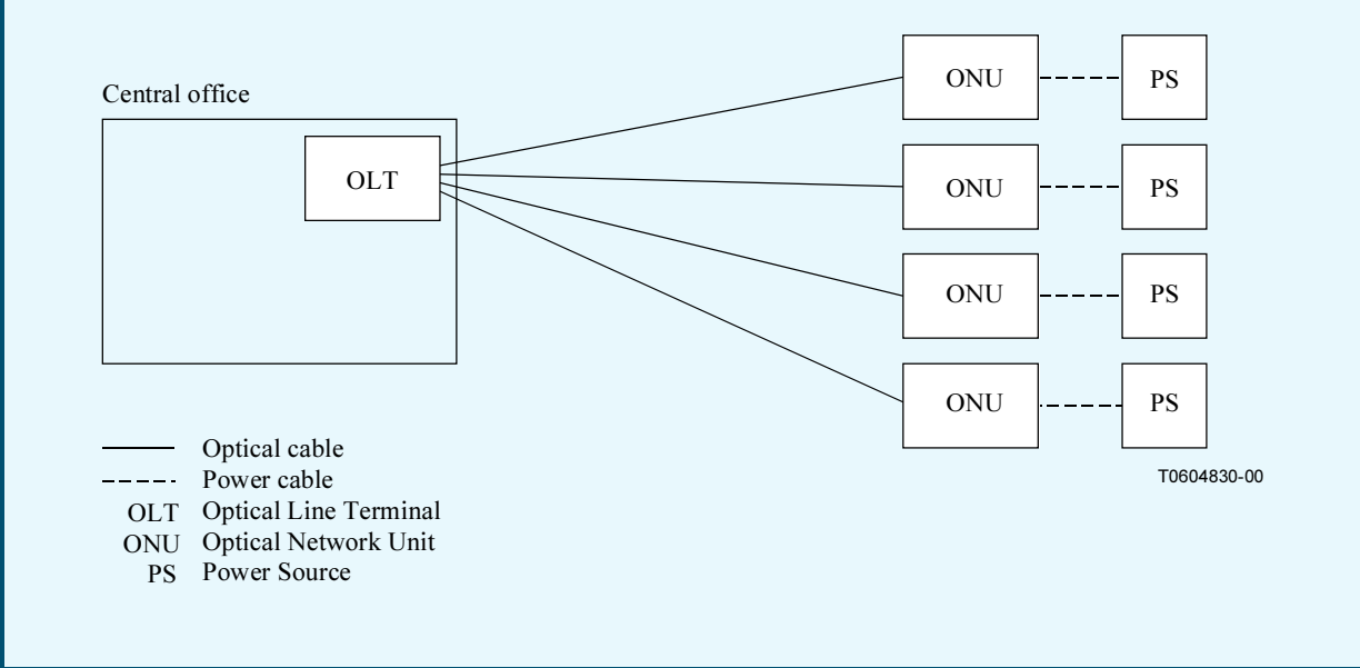
Figure 4-10: Individual power supply
