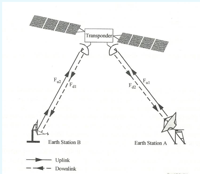
Figure 6-1: The basic satellite link
