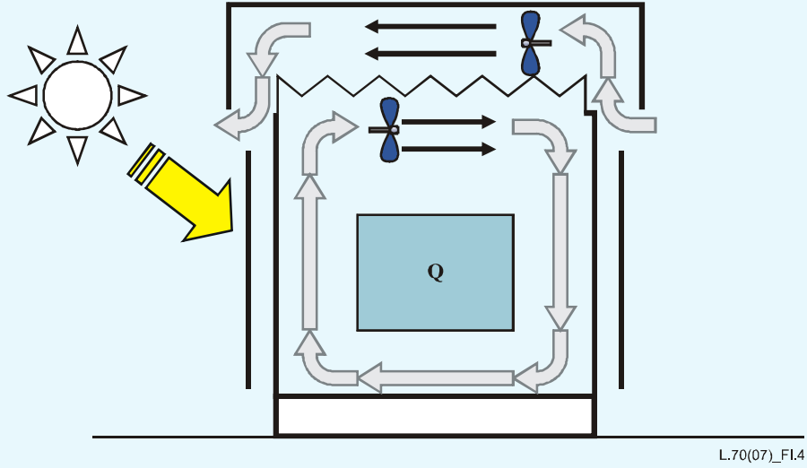
Figure 4A2-4: Dual wall, heat exchanger
