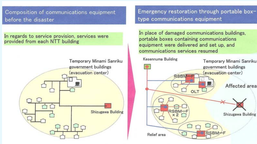
Figure 3-11: Emergency restoration of equipment
