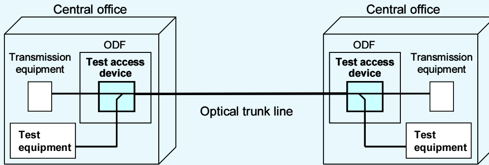
Figure 4-22: Typical configuration of an optical trunk line with test access devices
