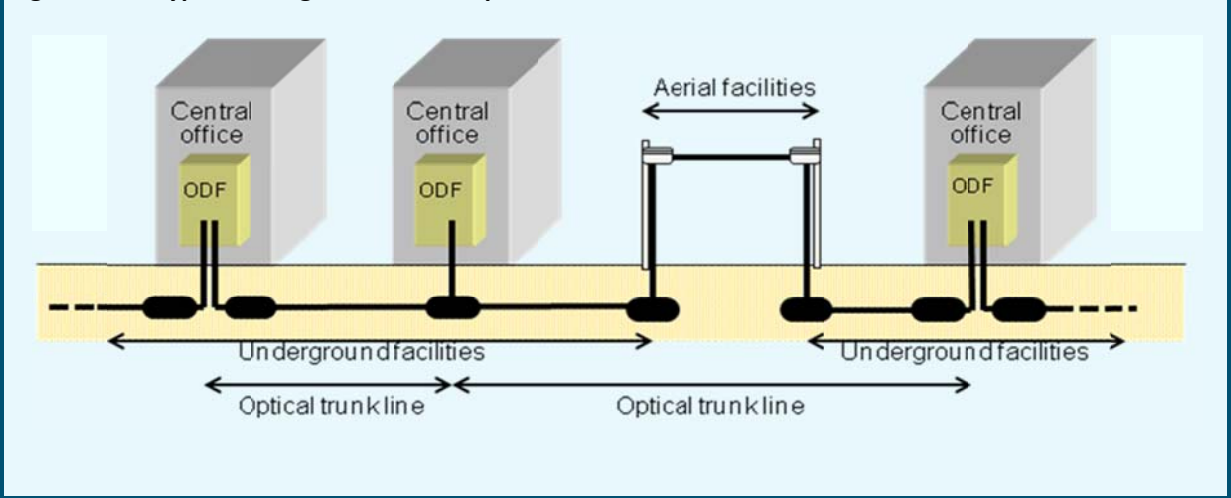
Figure 4-21: Typical configuration of an optical trunk line
