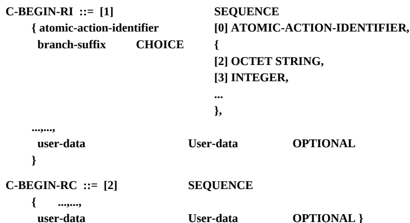
Figure 2 – C-BEGIN APDUs
