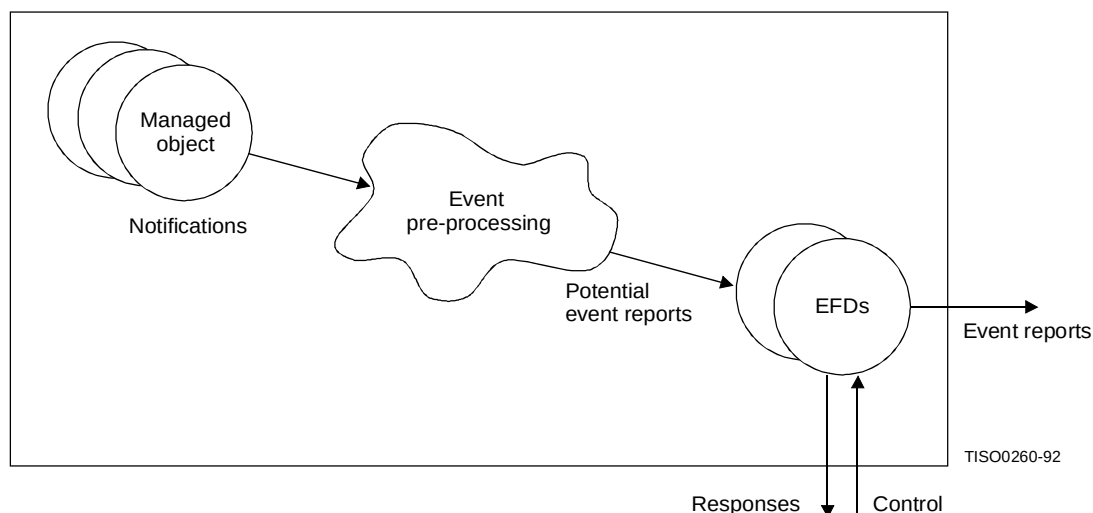
Figure 1 – Event report management model
