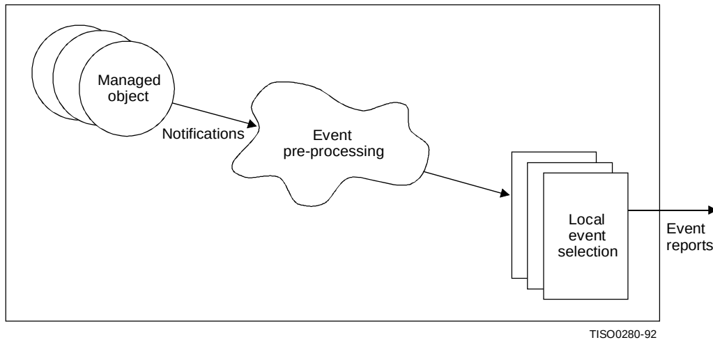
Figure B.1 – Local event selection mechanism
