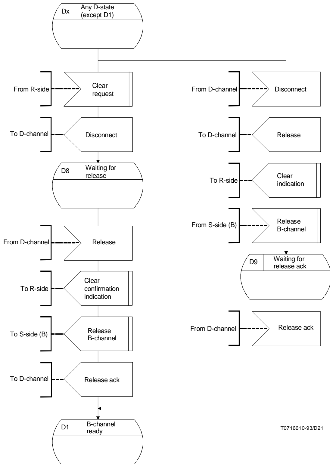
FIGURE A.5/X.30 S-interface side of the X.21 TA; clearing phase of the D-channel handler
