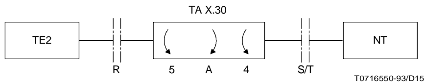
FIGURE 3-1/X.30 Location of test loops
