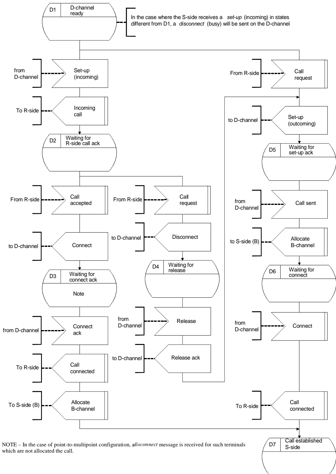
FIGURE A.4/X.30 S-interface side of the X.21 TA; call control phase of the D-channel handler
