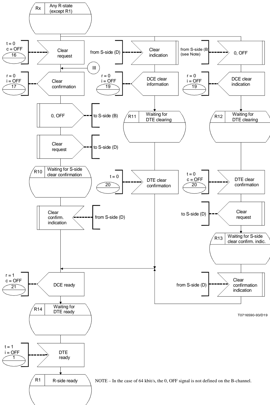
FIGURE A.3/X.30 R-interface side of the X.21 TA; clearing phase
