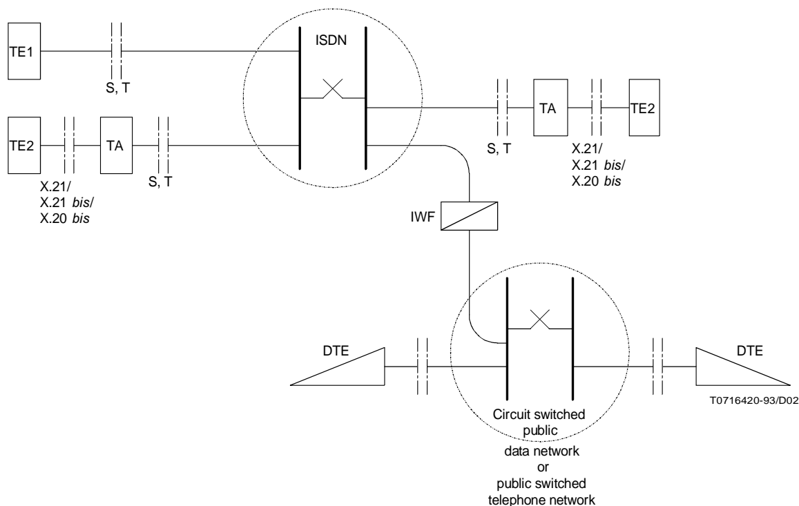
FIGURE 1-2/X.30 Network interworking configuration example
