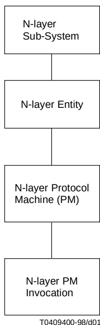
Figure 1 – Generic OSI Layer Containment Hierarchy
