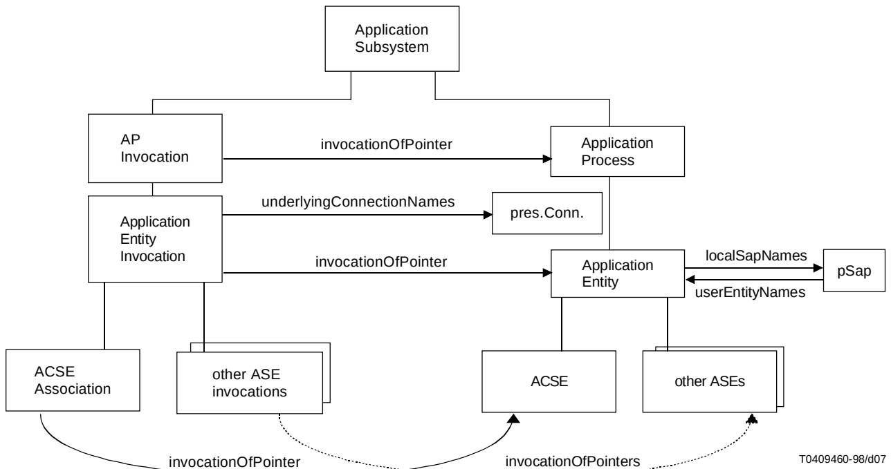
Figure 7 – Application Layer Containment Hierarchy with ACSE
