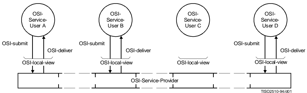
Figure 1 – OSI-service model
