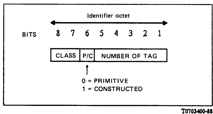
FIGURE 3/X.209 Identifier octet (low tag number)
