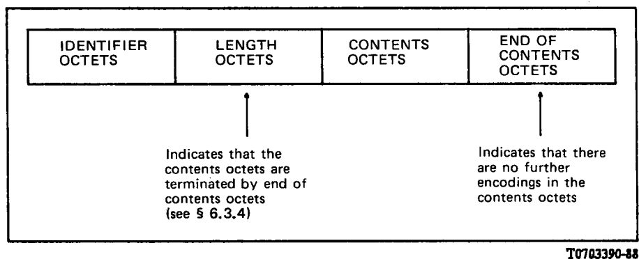
FIGURE 2/X.209 An alternative constructed encoding
