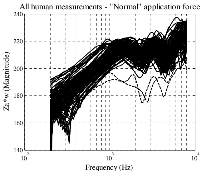
Figure I.4 – Impedance versus frequency bin line chart of the raw data (left plot) and the mean and sample standard deviation (right plot) for the normal application force case
