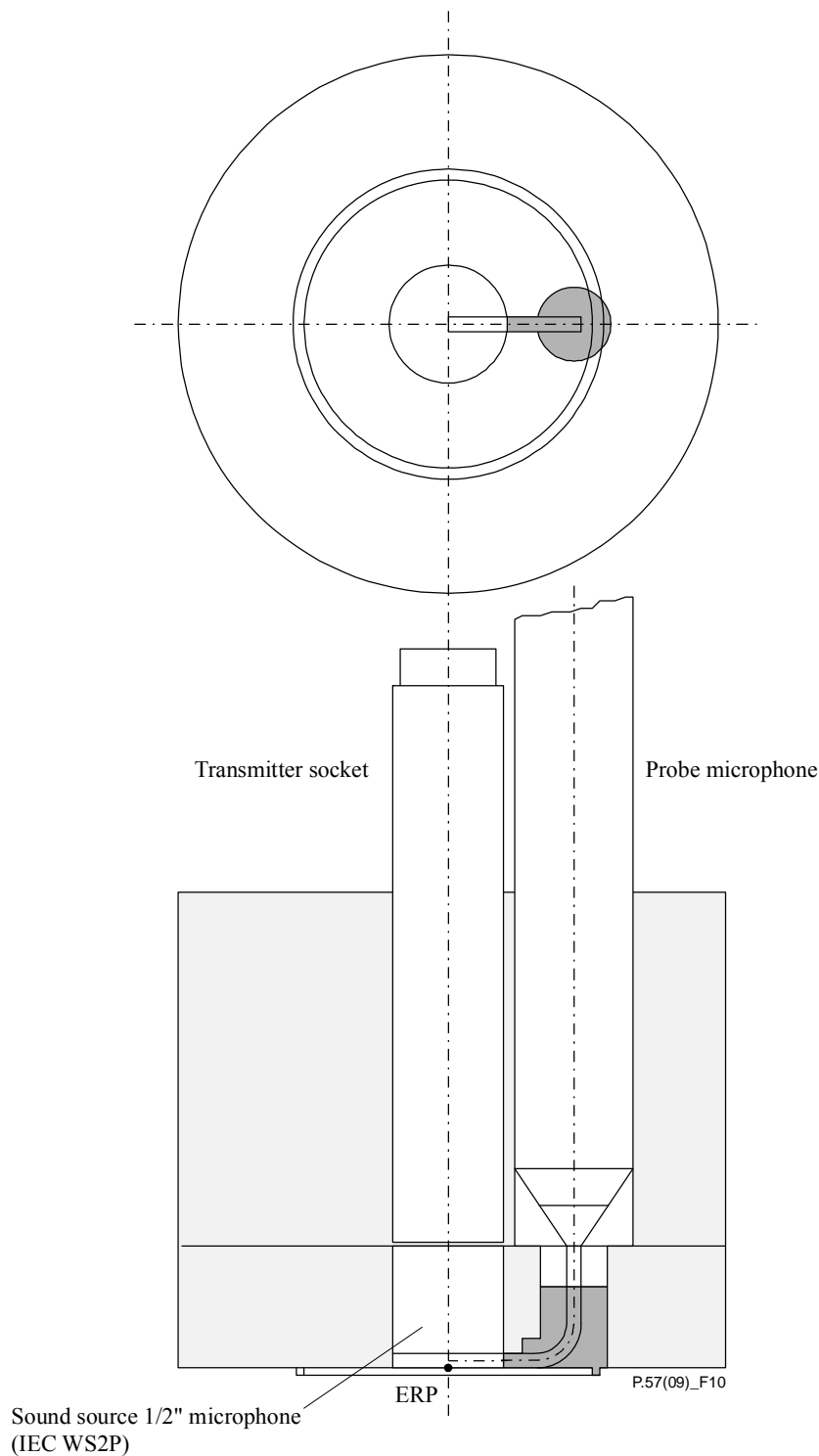
Figure 10 – Practical implementation of a calibration device (impedance probe) for measuring acoustical input impedance of type 1 and type 3.2 artificial ears
