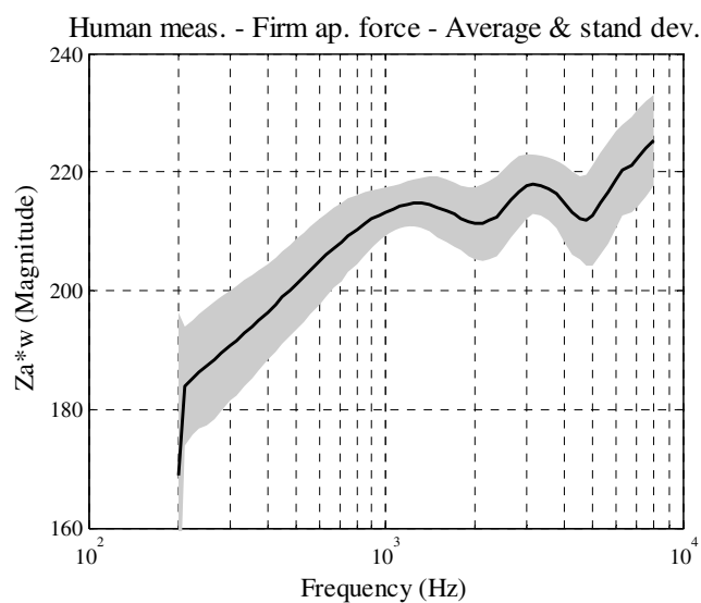
Figure I.5 – Impedance versus frequency bin line chart of the raw data (left plot) and the mean and sample standard deviation (right plot) for the firm application force case
