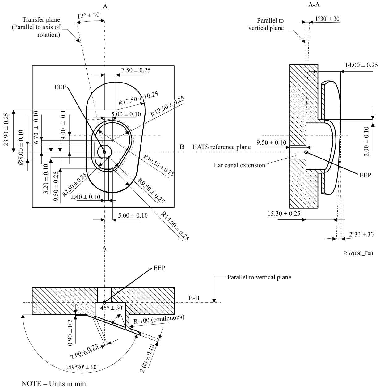
Figure 8 – Type 3.4 artificial ear
