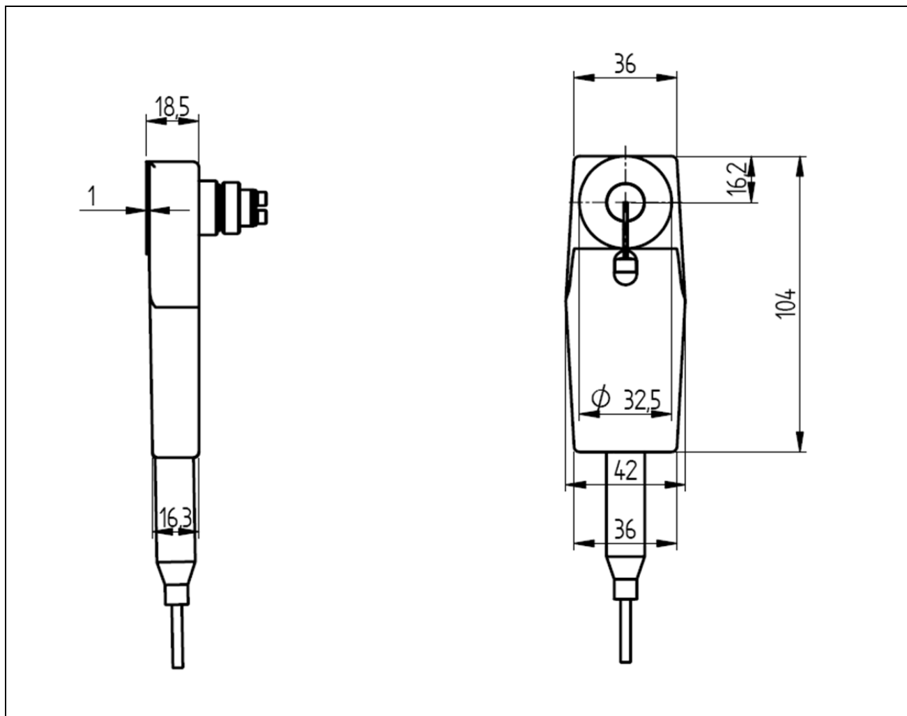
Figure II.1 – The mobile phone shaped impedance probe viewed from the side and from the front
