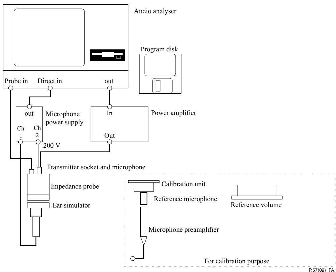
Figure A.1 – Measurement set-up
