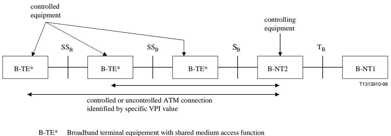
Figure 3/I.150 – GFC at the multi-access UNI
