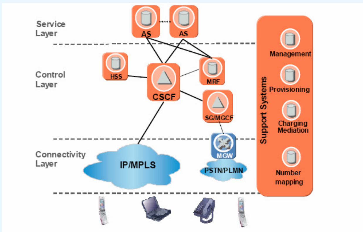
Figure 6.2: IMS Architecture
