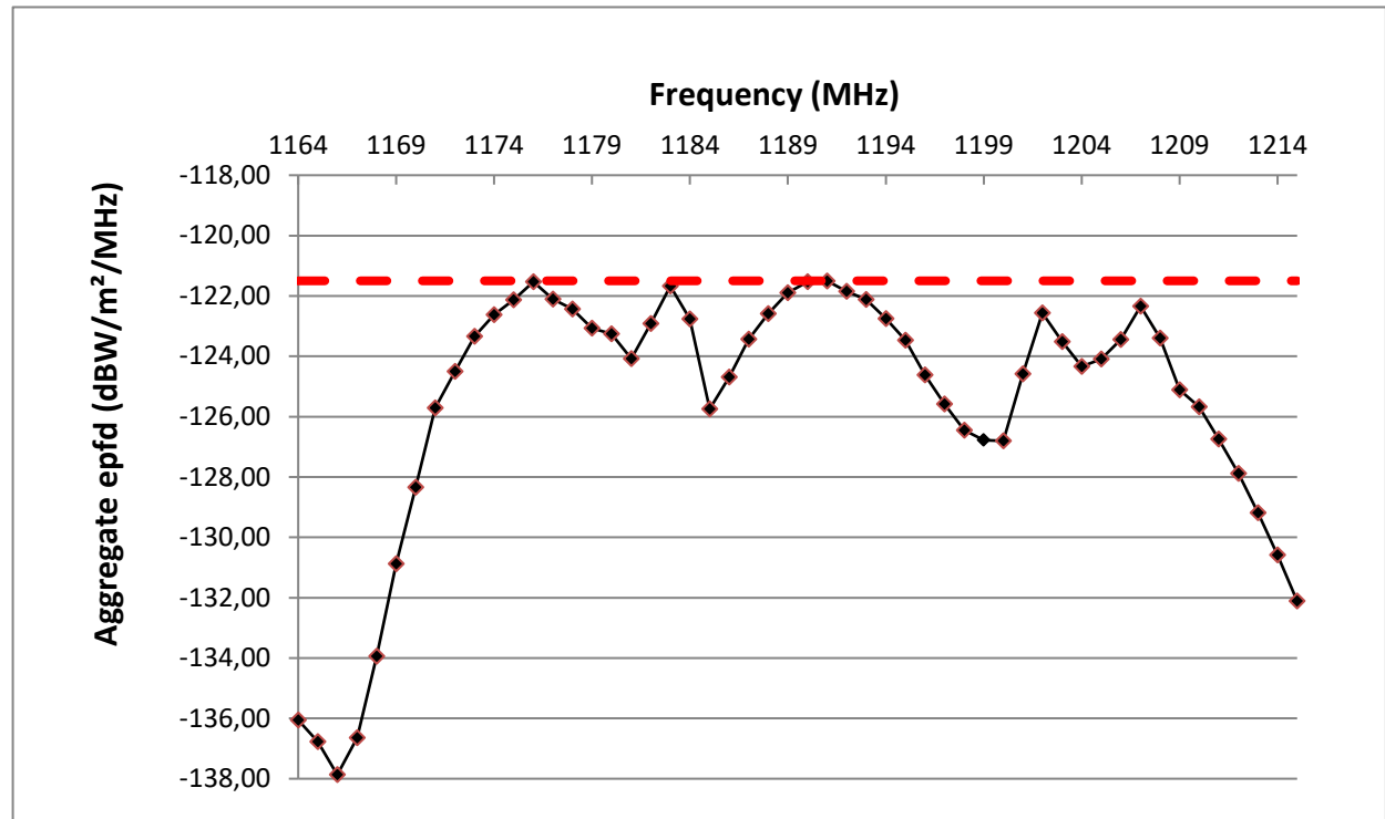
Figure 2: Plot of Table 3 (Maximum RNSS Aggregate epfd per MHz) for case 4
