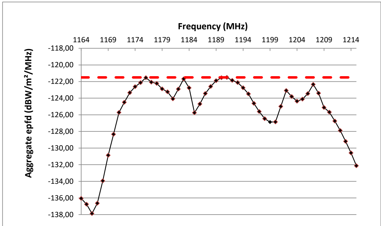
Figure 1: Plot of Table 2 (Maximum RNSS Aggregate epfd per MHz) for case 1
