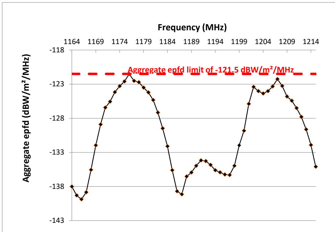
Figure 1: Plot of Table 2 (Maximum RNSS Aggregate epfd per MHz) for case 1
