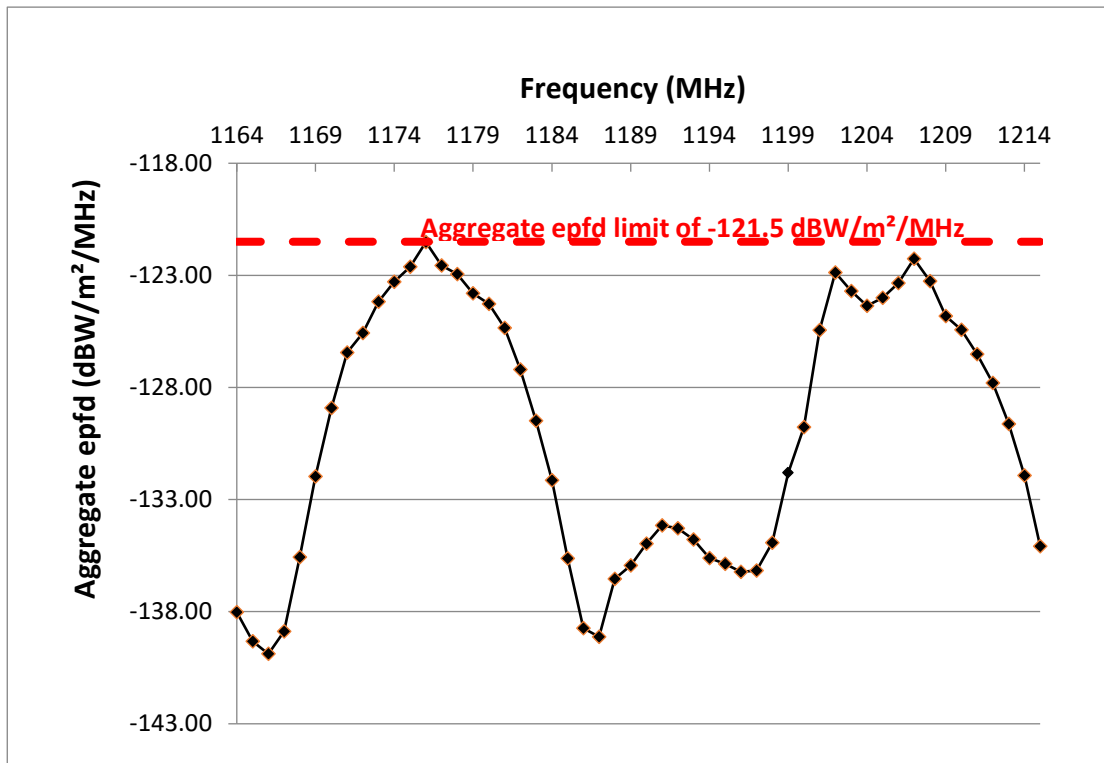
Figure 2: Plot of Table 3 (Maximum RNSS Aggregate epfd per MHz) for case 2
