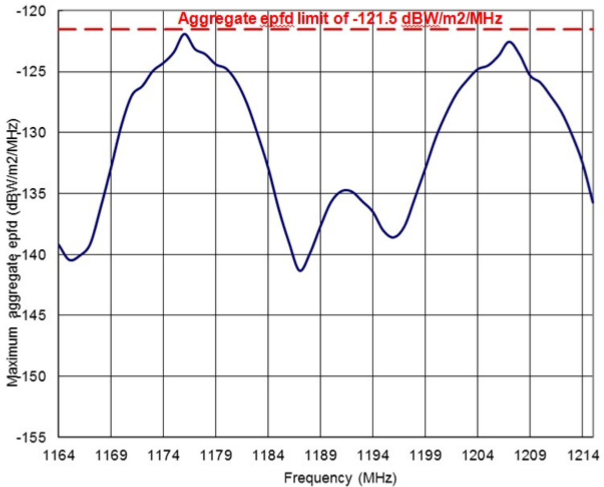
Figure 1: Plot of Table 3 (Maximum RNSS Aggregate epfd per MHz)
