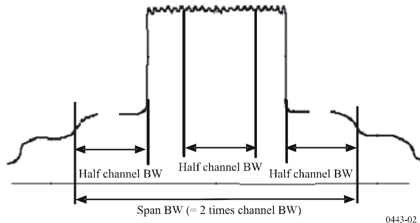
FIGURE 2 ACPR using half channel bandwidth
