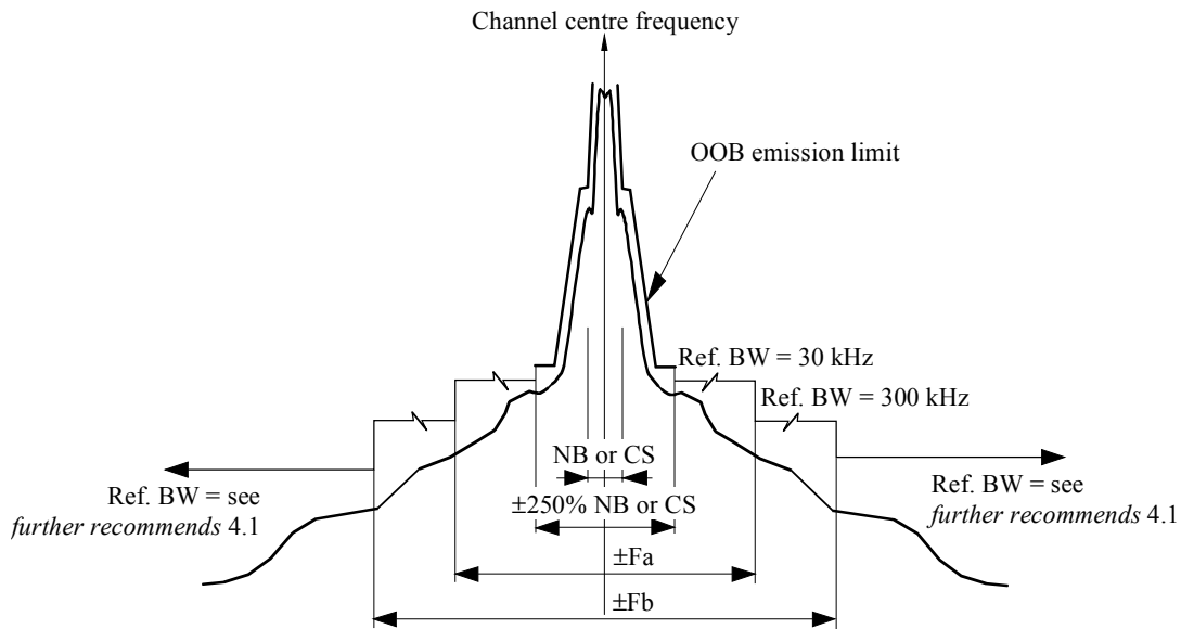
FIGURE 5 Generic spurious emission mask for Category B land mobile service stations (refer to Table 13)
