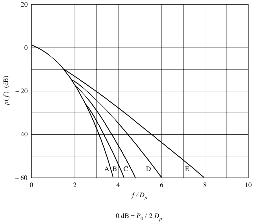
FIGURE 8 Power spectral distribution for D_p/M > 0.5
