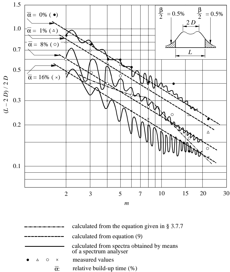
FIGURE 7 Comparison of the results of calculations and measurements of occupied bandwidth
