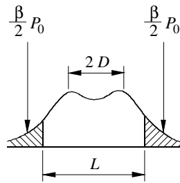
Bandwidth calculation from the empirical formula (8)
