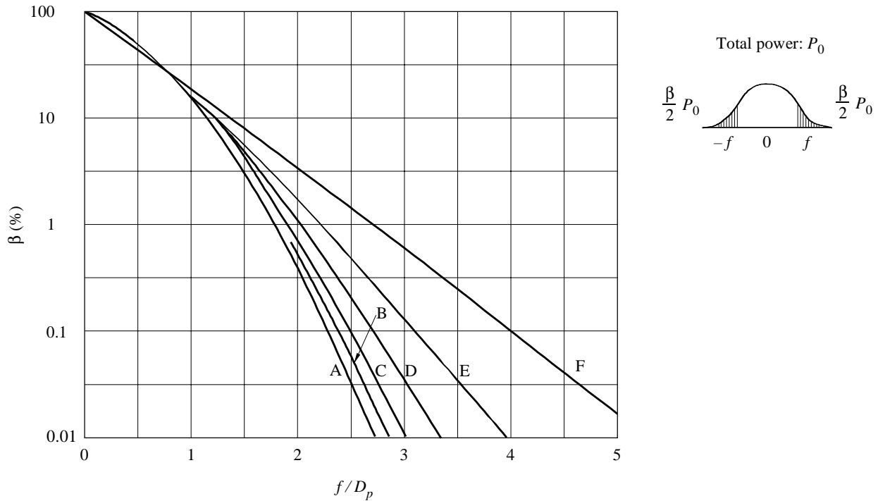
FIGURE 10 Out-of-band power of the spectra for D_p/M > 0.5
