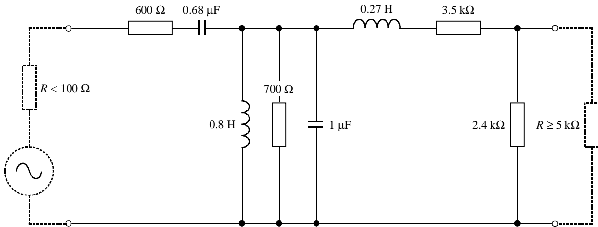
Filter circuit
