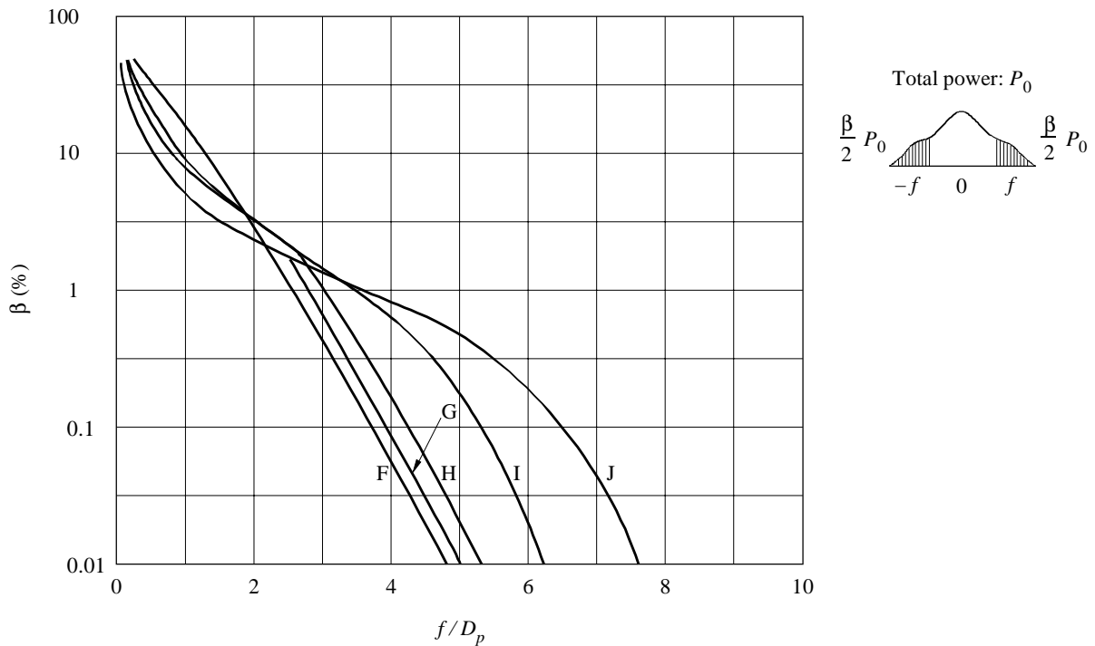
FIGURE 11 Out-of-band power of the spectra for D_p/M < 0.5
