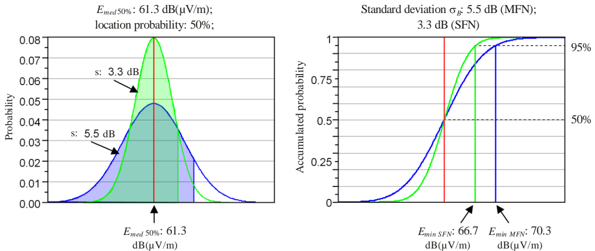
FIGURE 3 Network gain
