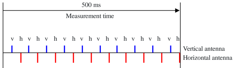
FIGURE 11 Measurement timing for SFNs with mixed polarization (portable reception)
