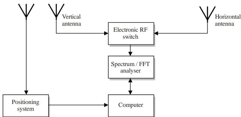
FIGURE 9 Measurement setup (portable reception inside SFNs)
