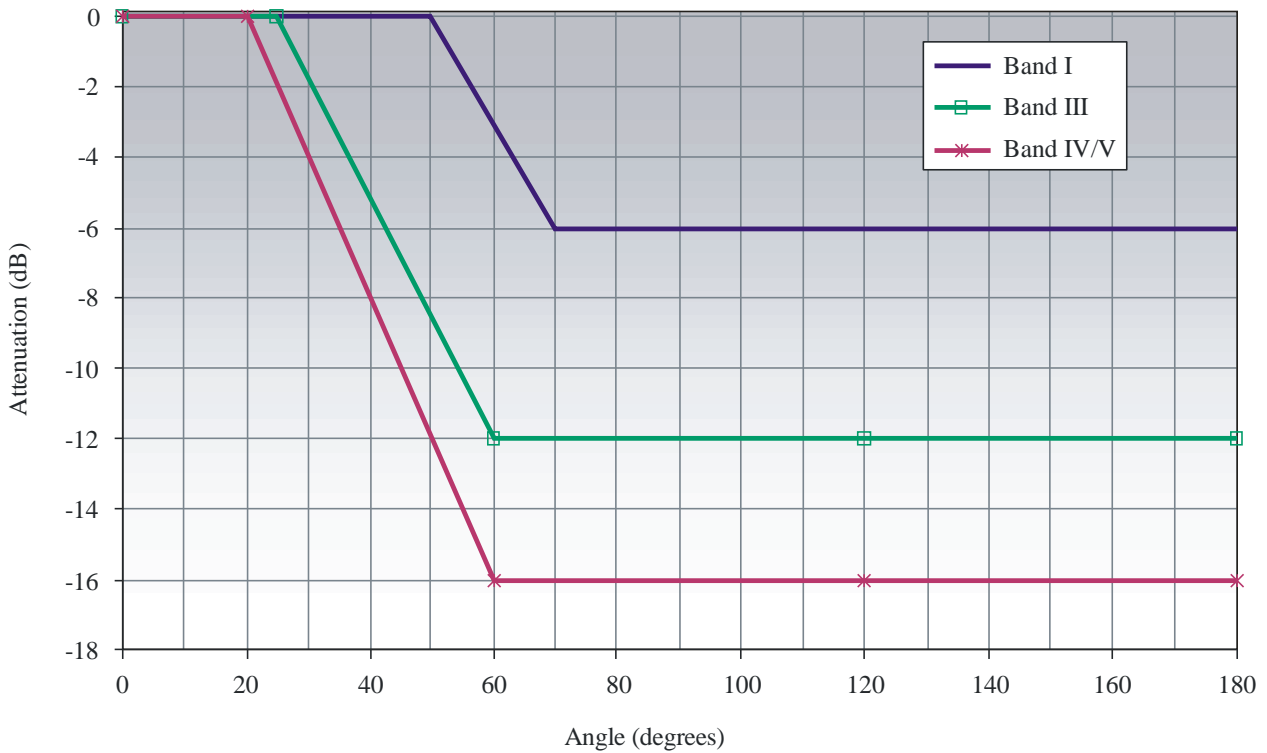
Relative antenna directivity for fixed broadcast reception
