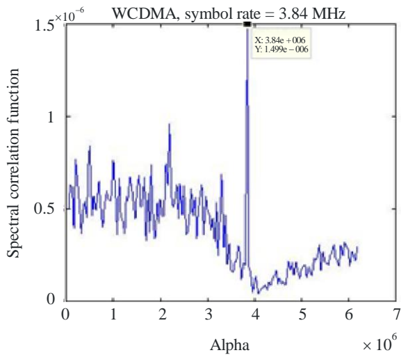
a) Estimation of symbol rate
