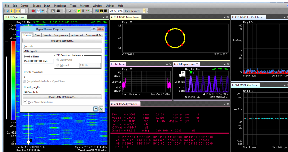
FIGURE 7C GSM Uplink Analysis Results
