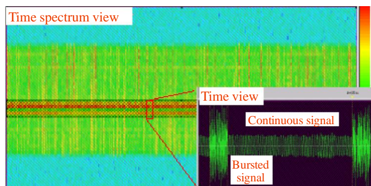
Time and spectrum diagram (Frequency/Amplitude on Y-axis and time on x-axis):
