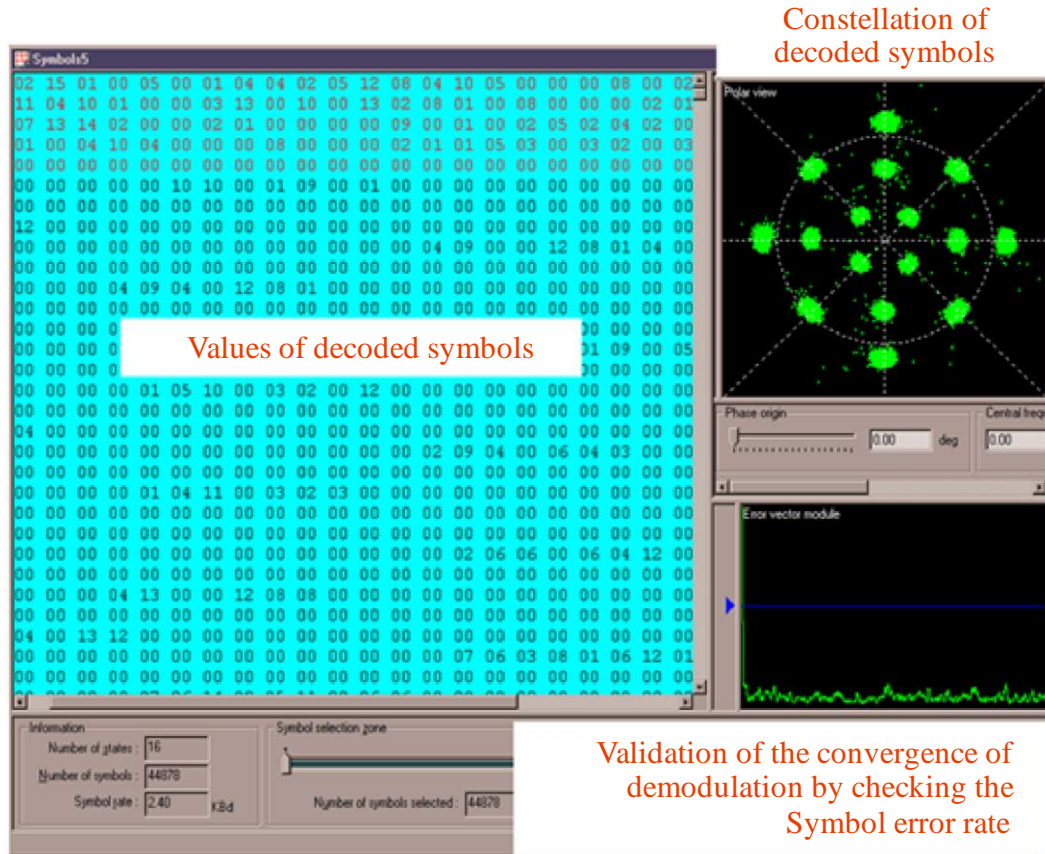
FIGURE 10 Example of demodulated 16QAM V29 signal
