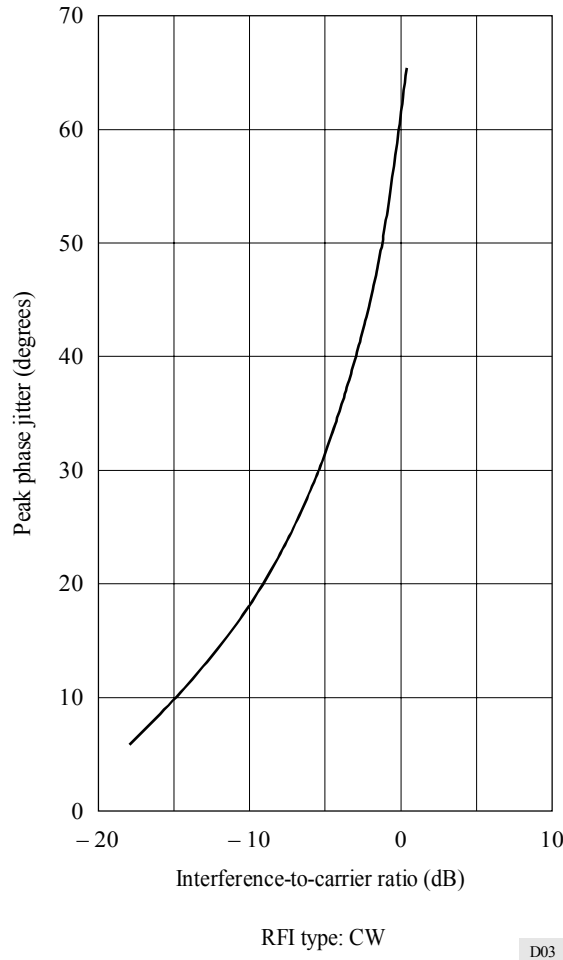
FIGURE 3 Peak phase jitter interference-to-carrier ratio
