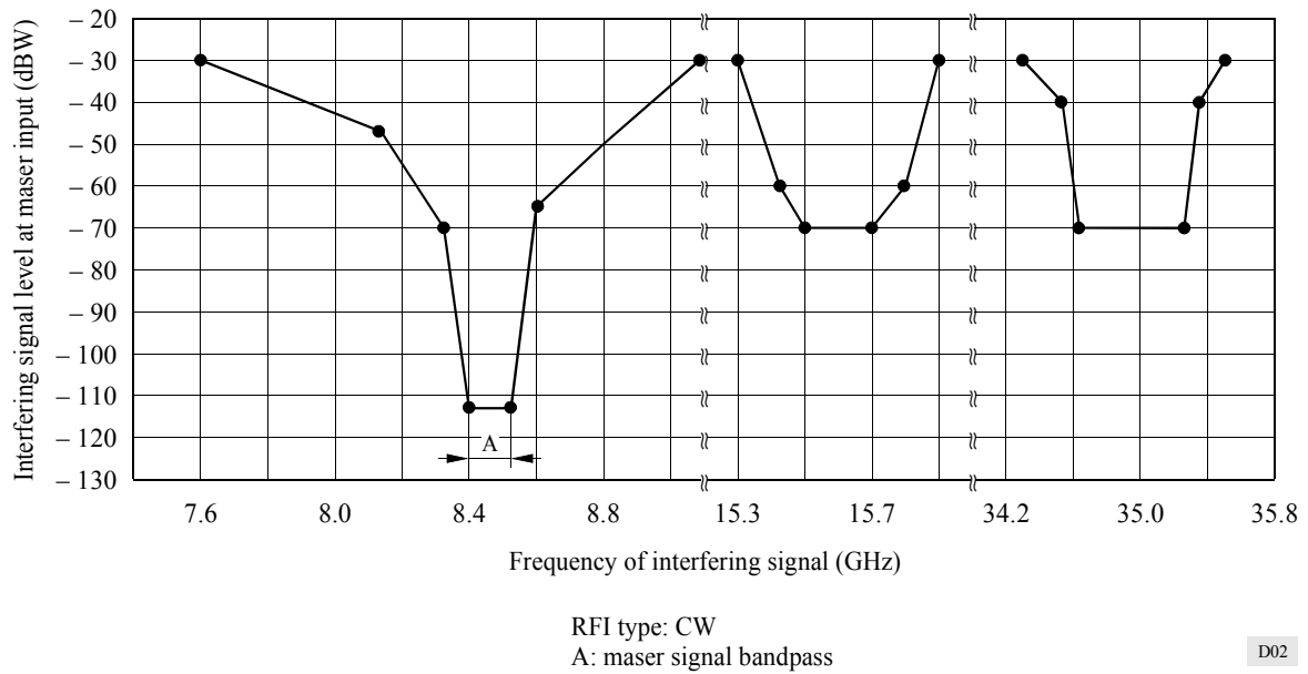
FIGURE 2 Signal level required to reduce the gain of a 8.45 GHz maser by 1 dB, versus frequency
