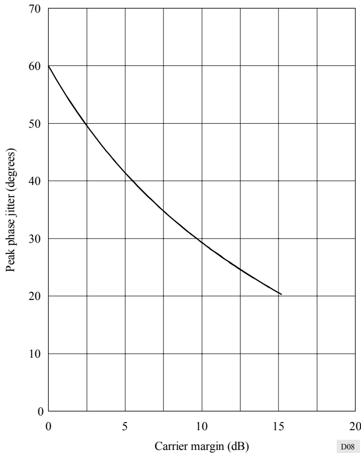
FIGURE 8 Peak phase jitter versus carrier margin
