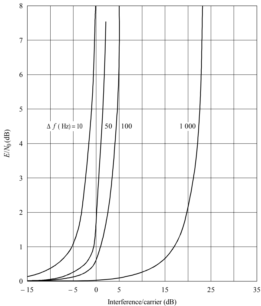
FIGURE 6 Equivalent reduction in ranging signal-to-noise ratio, E/N_0 , as a result of carrier loop phase error and jitter versus interference-to-carrier ratio, for selected values of frequency offset
