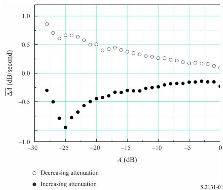
Average fading slope in a Ka band satellite system
