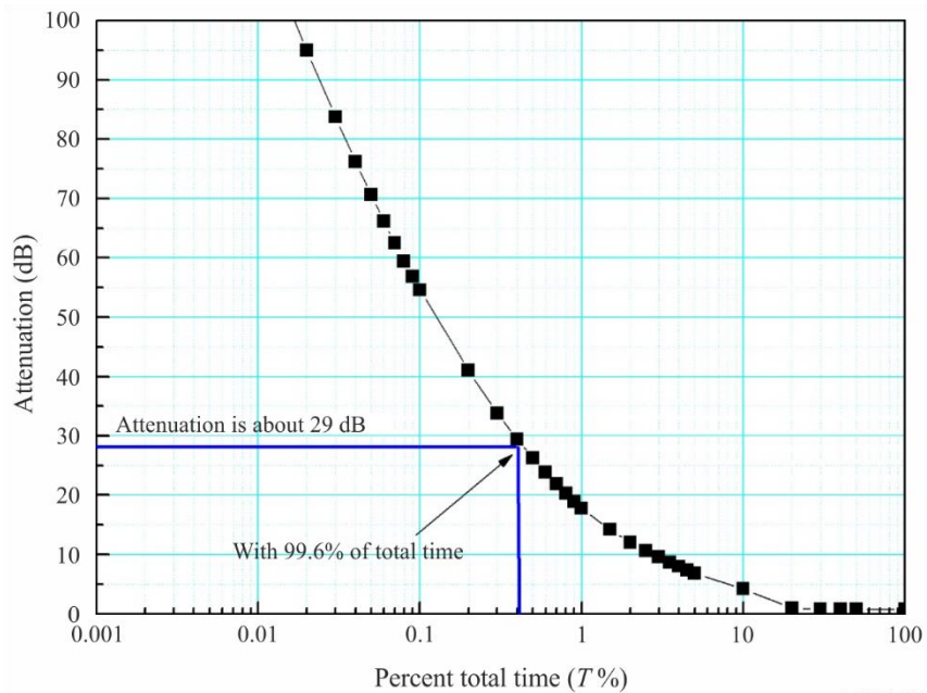
Attenuation due to propagation loss based on Recommendation ITU-R P.618 for a satellite connection utilizing ACM and operating in a climatological area similar to South Florida, USA
