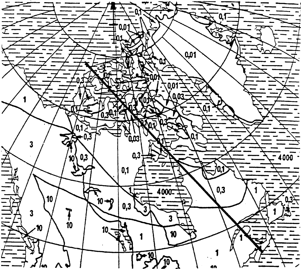
FIGURE 31 VLF ground conductivity map for Canada and the Arctic (mS/m)
