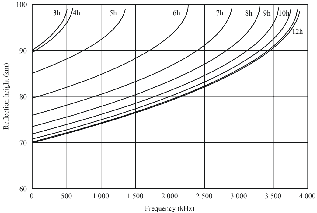
Variation in the height of reflection layer with local time
