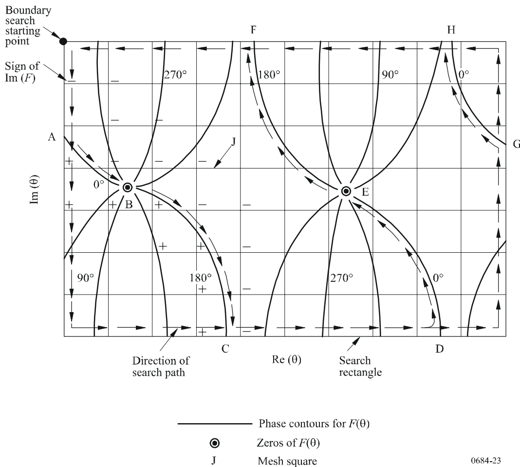
FIGURE 23 Mode finding method for the function F(\theta)
