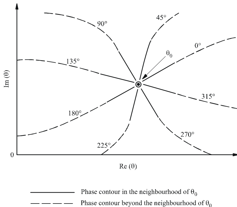
FIGURE 22 Phase contour behaviour near a zero of F(\theta)
