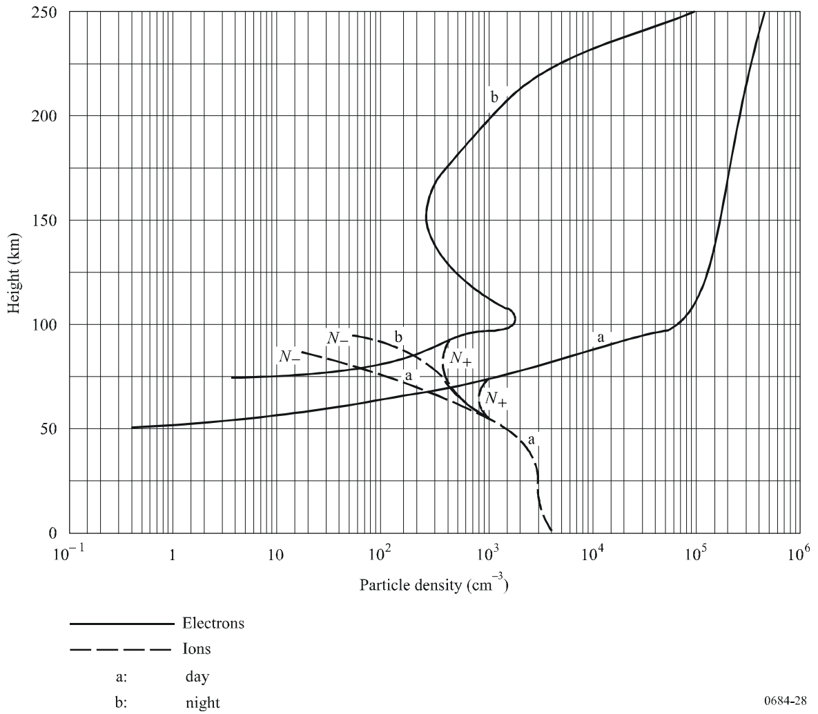
FIGURE 28 Ambient day and night constituent profiles
