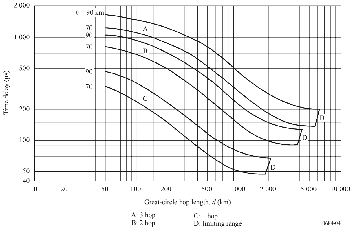
FIGURE 4 Differential time delay between surface wave and one, two and three hop sky waves
