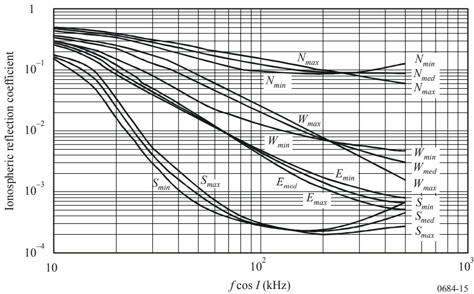
FIGURE 15 Ionospheric reflection coefficient
