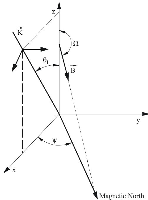
FIGURE 21 Wave propagation geometry
