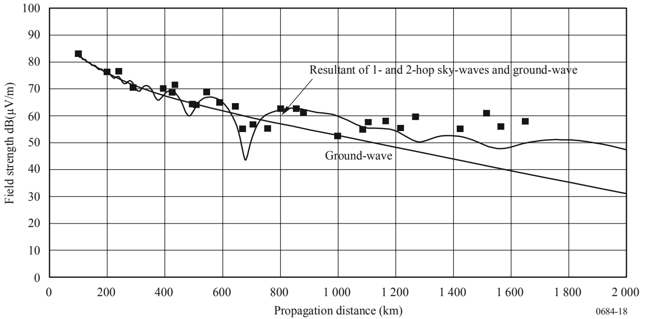
FIGURE 18 Field strengths of JJY 60 kHz wave received in the daytime in February 2004
