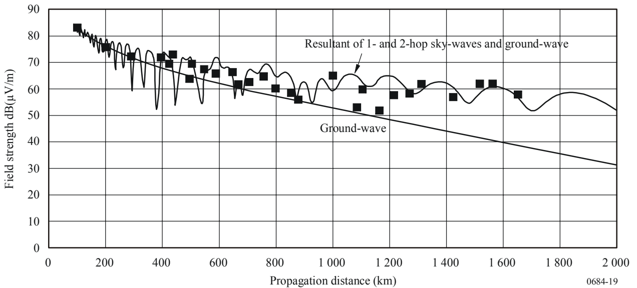
FIGURE 19 Field strengths of JJY 60 kHz wave received at night-time in February 2004
