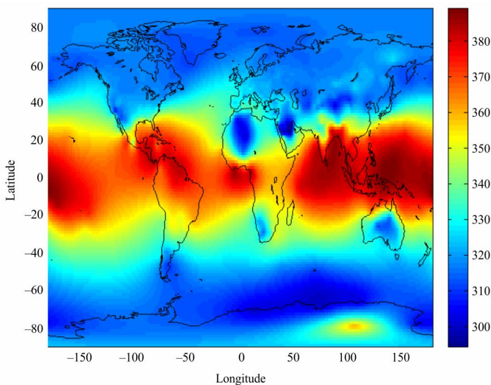
FIGURE 1 Average annual sea-level surface refractivity, N_0
