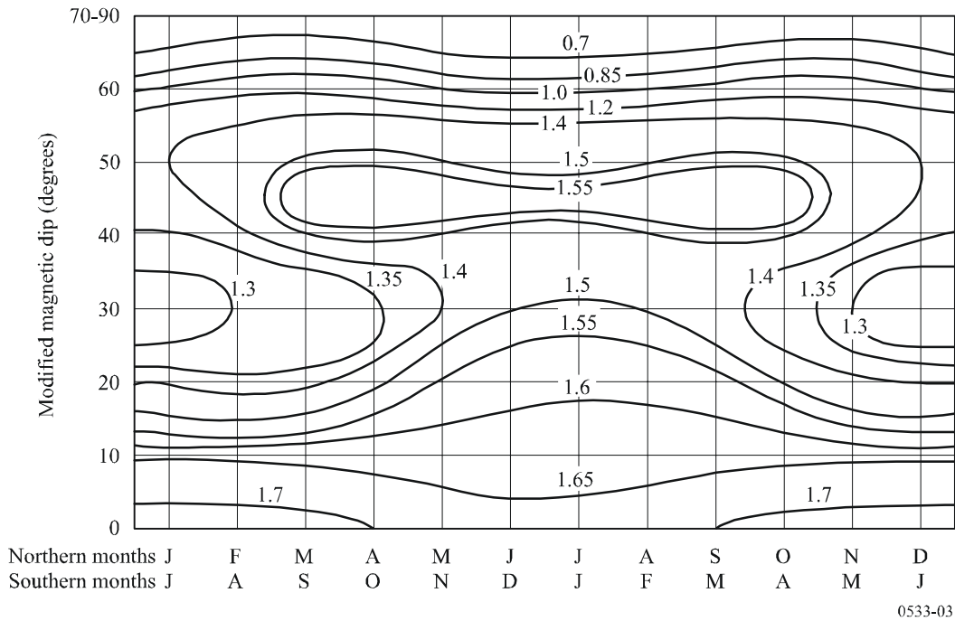
The diurnal absorption exponent, p
