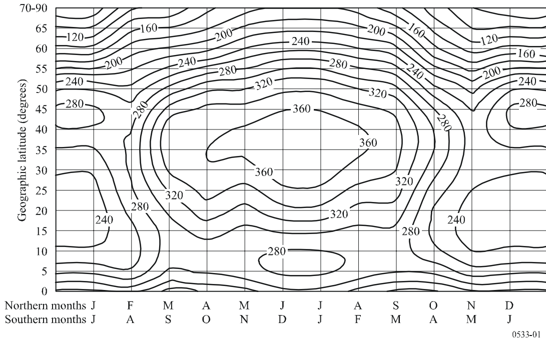
FIGURE 1 The absorption factor, AT_{noon}
