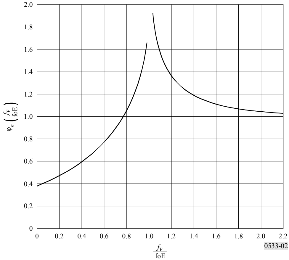
FIGURE 2 The absorption layer penetration factor, \phi_n \left( \frac{f_y}{foE} \right)
