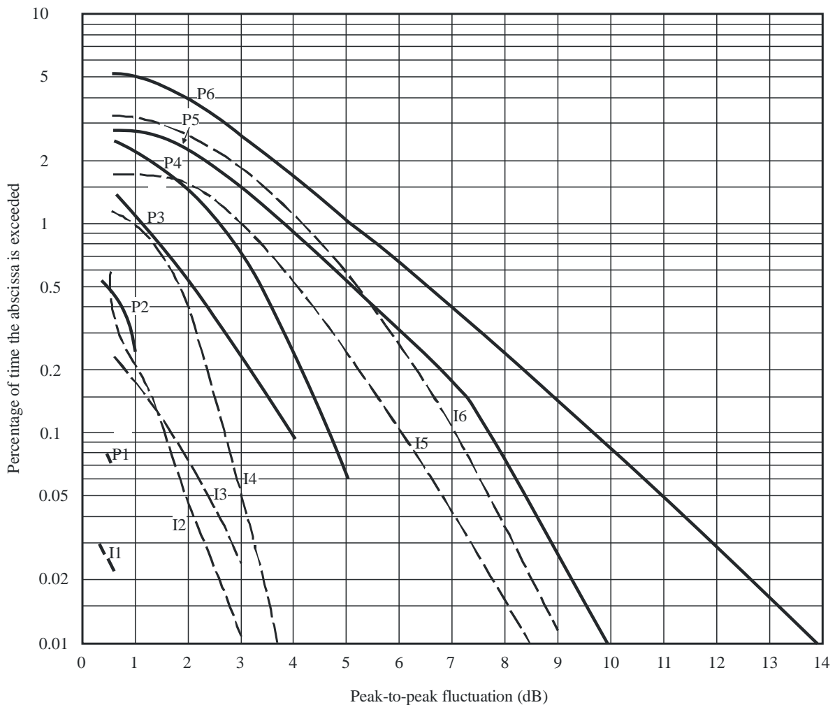
FIGURE 12 Annual statistics of peak-to-peak fluctuations observed at Hong Kong earth station (Curves I1, P1, I3-16, P3-P6) and Taipei earth station (Curves P2 and I2)
