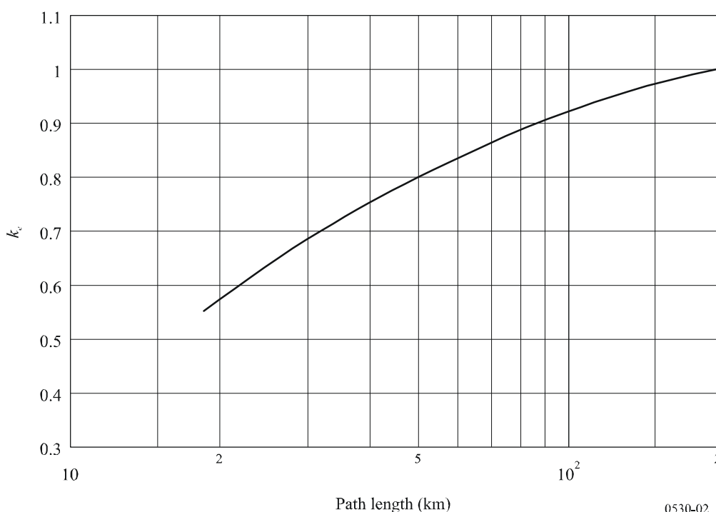
FIGURE 2 Value of k_e exceeded for approximately 99.99% of the worst month (continental temperature climate)
