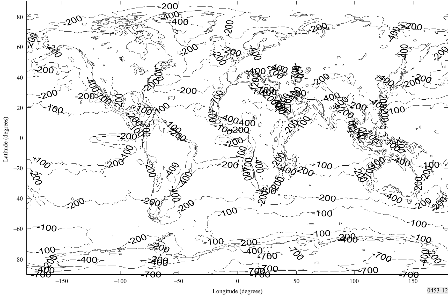
FIGURE 12 Refractivity gradient not exceeded for 1% of the average year in the lowest 65 m
