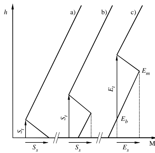
FIGURE 17 Definition of parameters describing a) surface, b) elevated surface and c) elevated ducts
