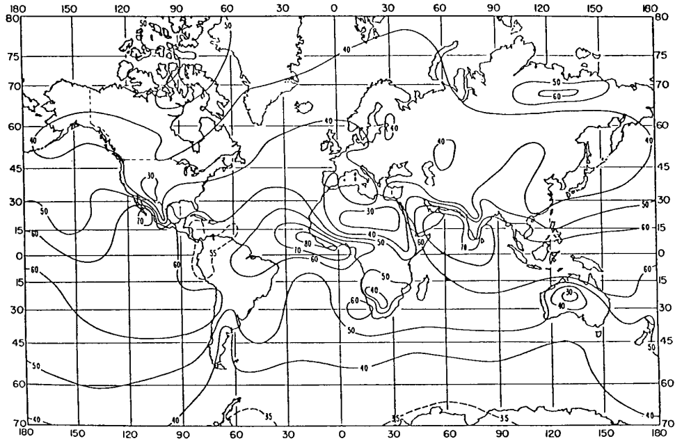
FIGURE 4 Monthly mean values of \Delta N : February
