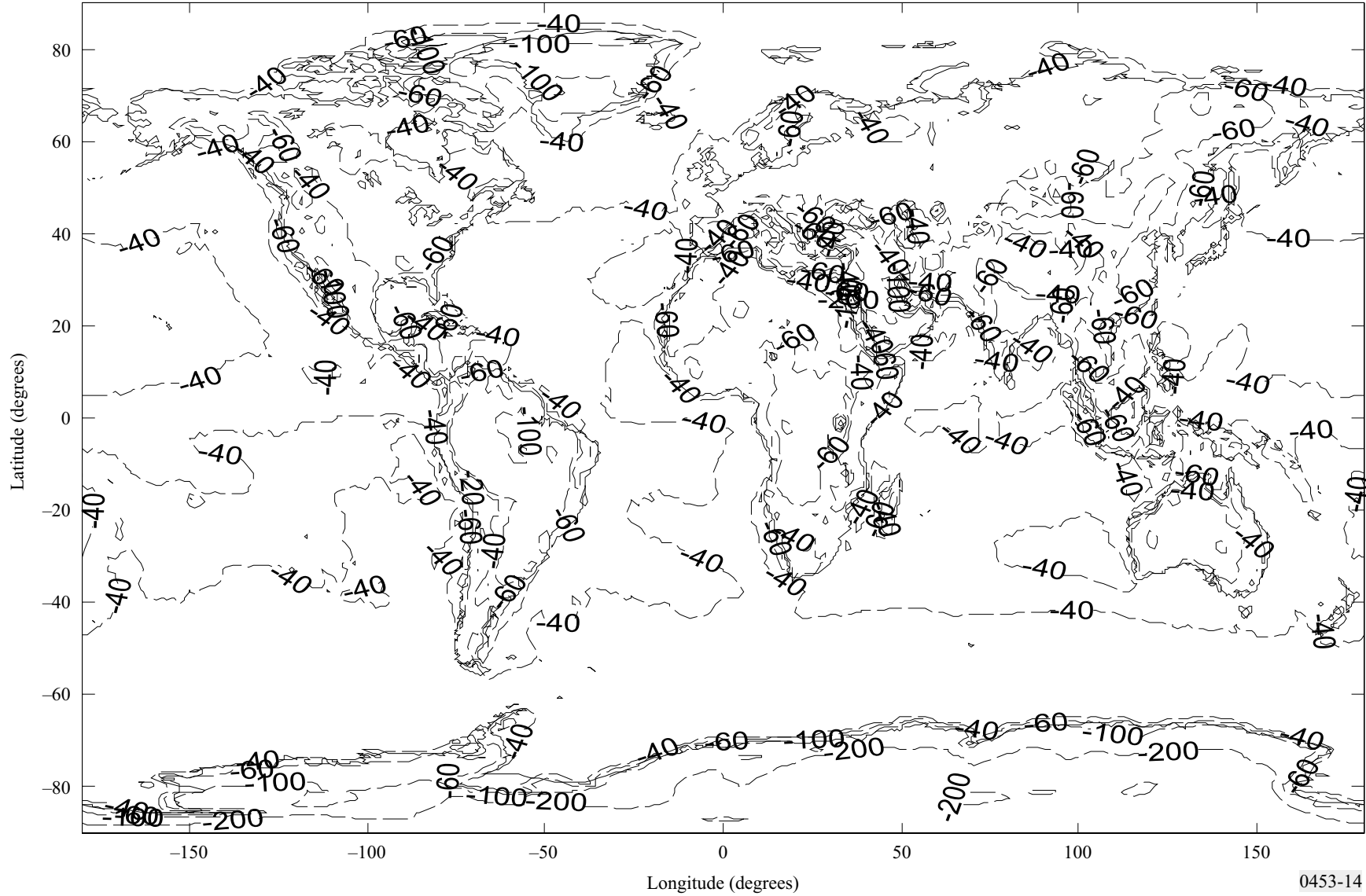
FIGURE 14 Refractivity gradient not exceeded for 50% of the average year in the lowest 65 m
