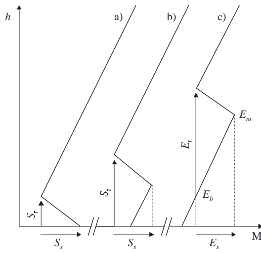
FIGURE 17 Definition of parameters describing a) surface, b) elevated surface and c) elevated ducts
