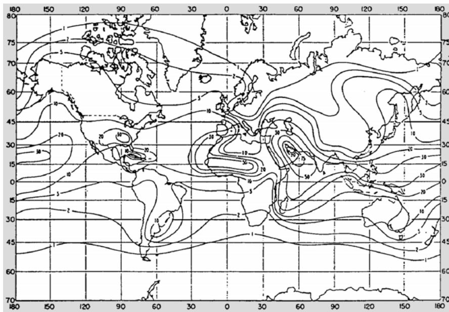
FIGURE 10 Percentage of time gradient \leq -100 (N-units/km): August
