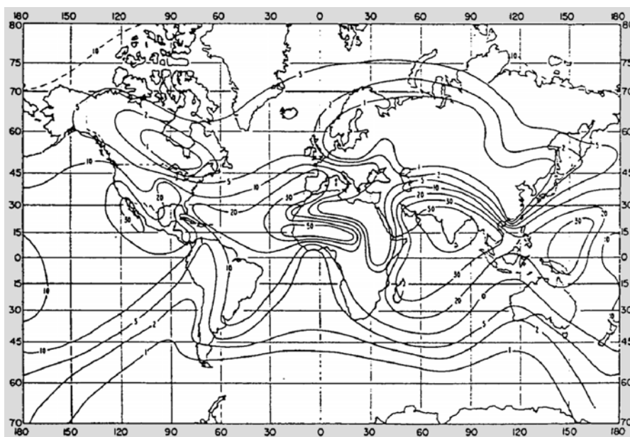
FIGURE 11 Percentage of time gradient \leq -100 (N-units/km): November
