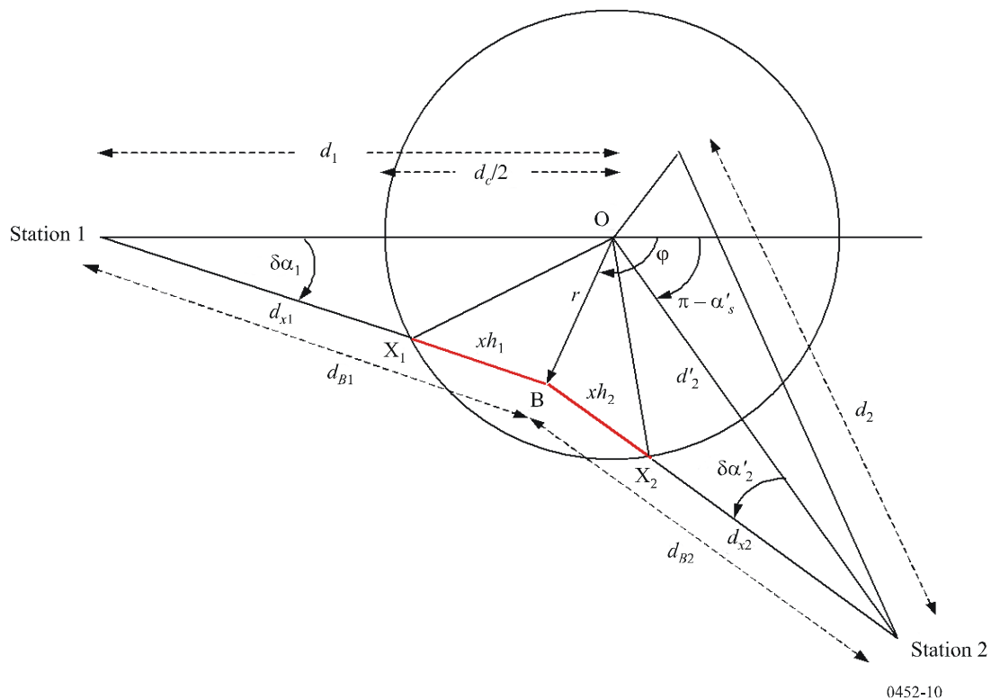
Plan view of scatter geometry through the integration element
