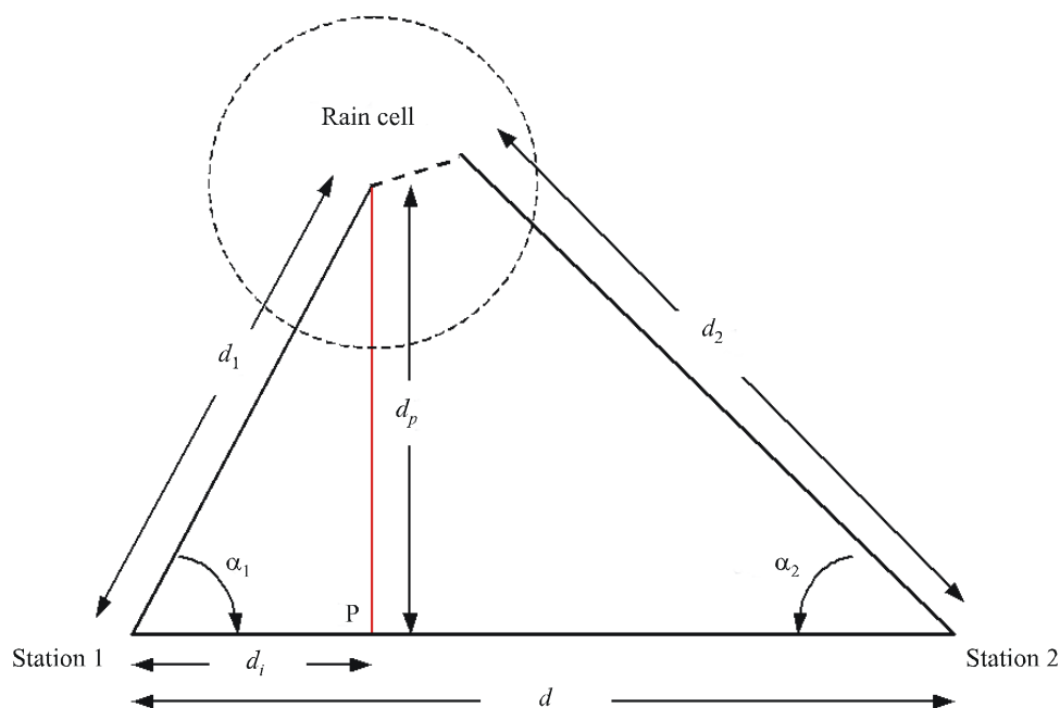
Plan view of geometry for side scattering
