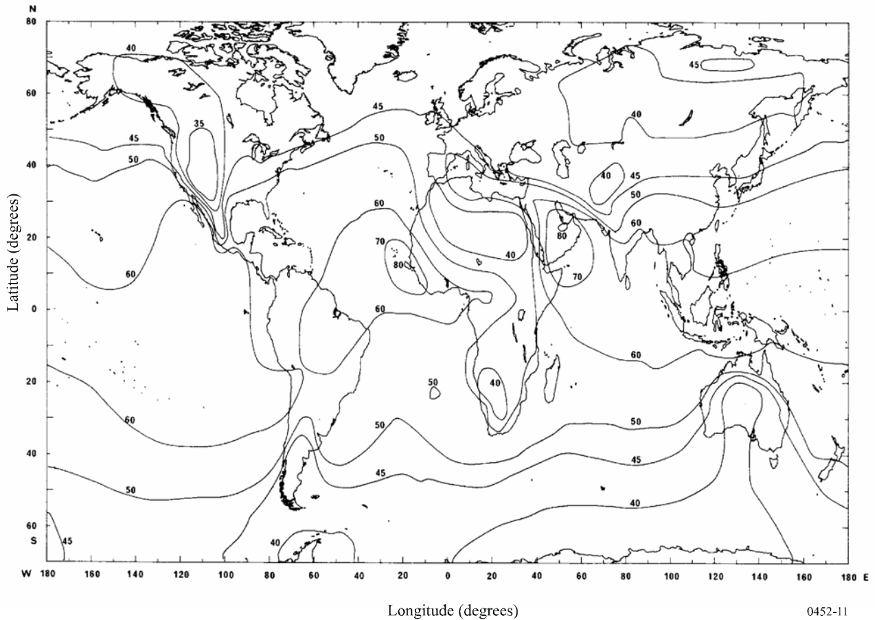
FIGURE 11 Average annual values of \Delta N
