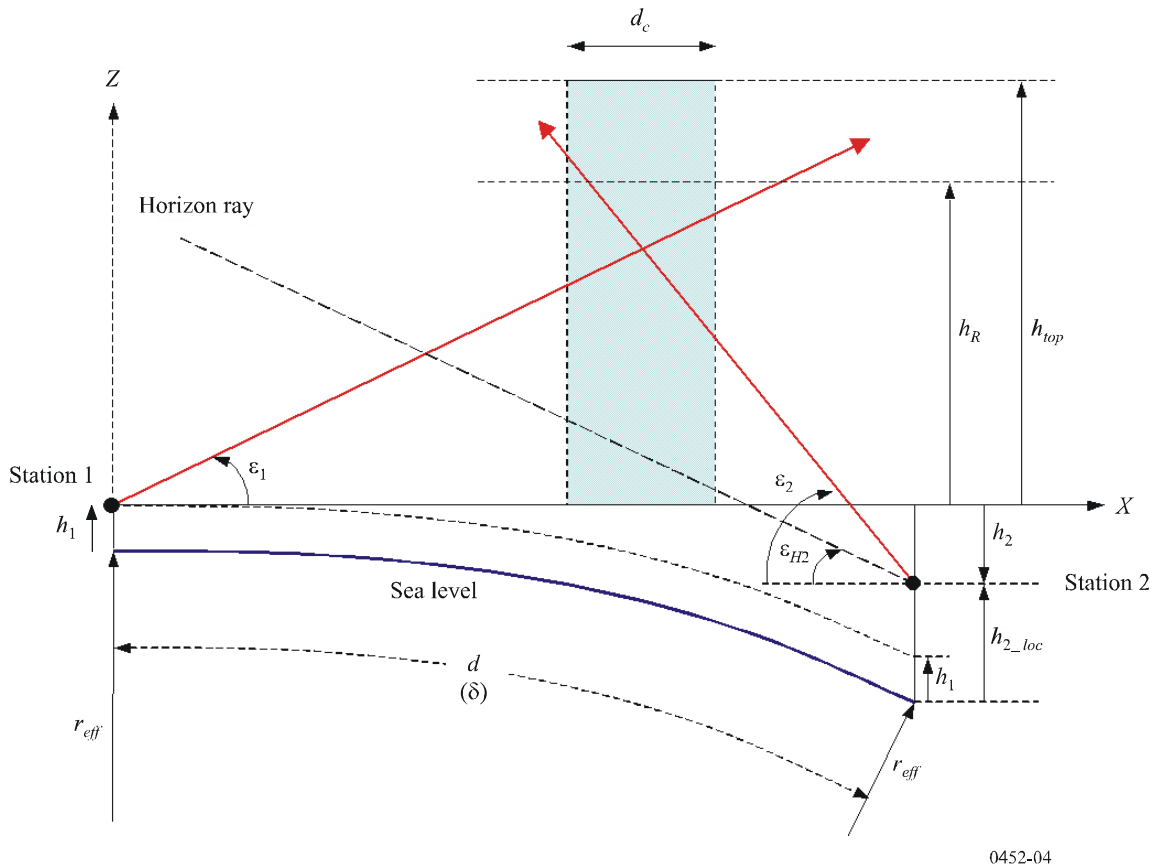
FIGURE 4 Geometry of stations on curved Earth
