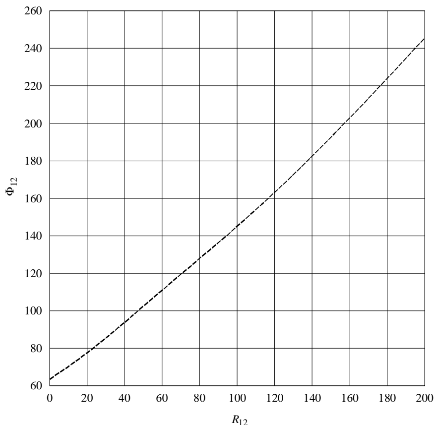
FIGURE 1 Relation entre R_{12} et \Phi_{12}
