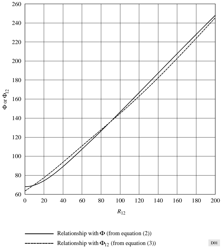
FIGURE 1 Relationship between R_{12} and \Phi or \Phi_{12}
