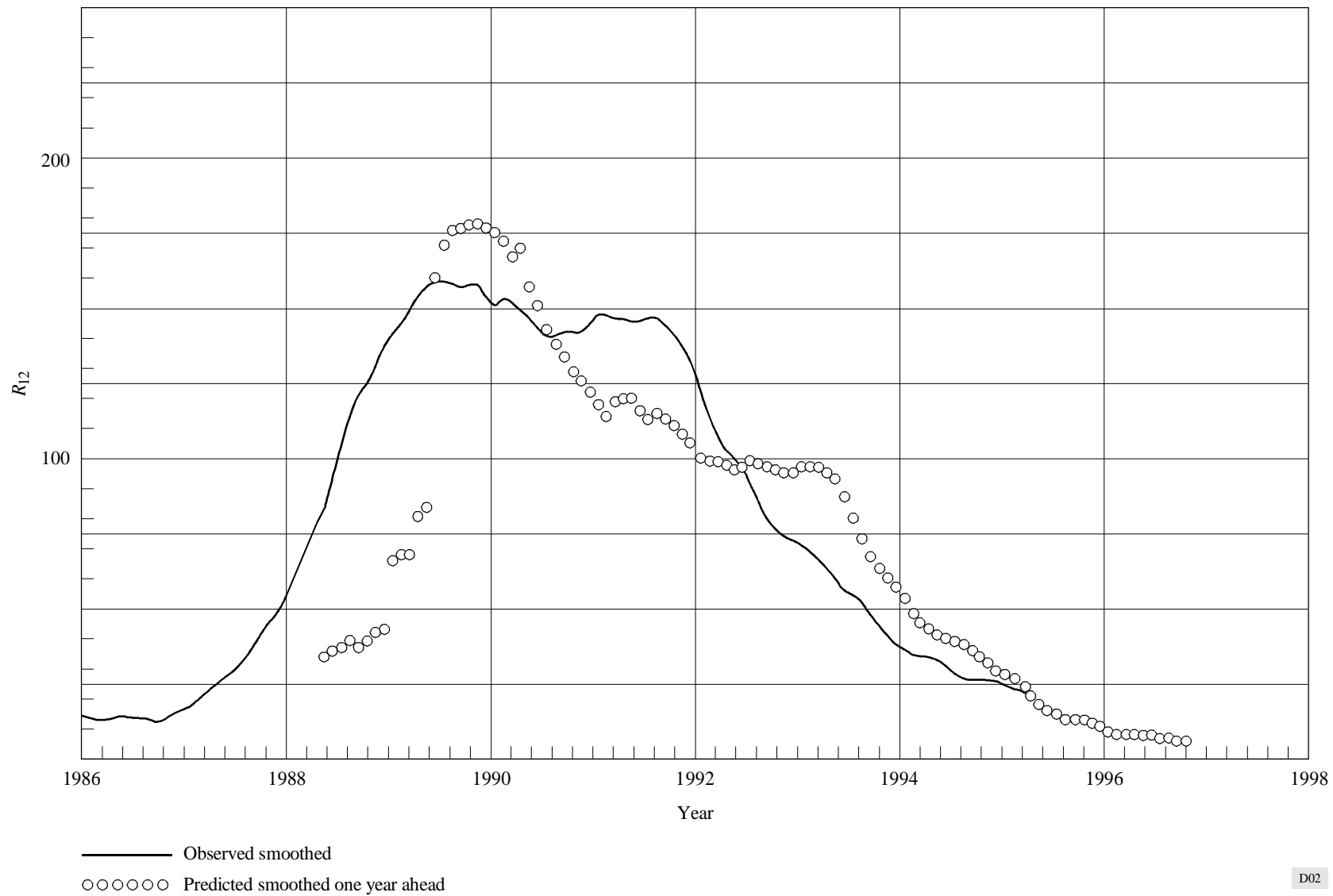
FIGURE 2 Predicted and observed sunspot numbers, R_{12}
