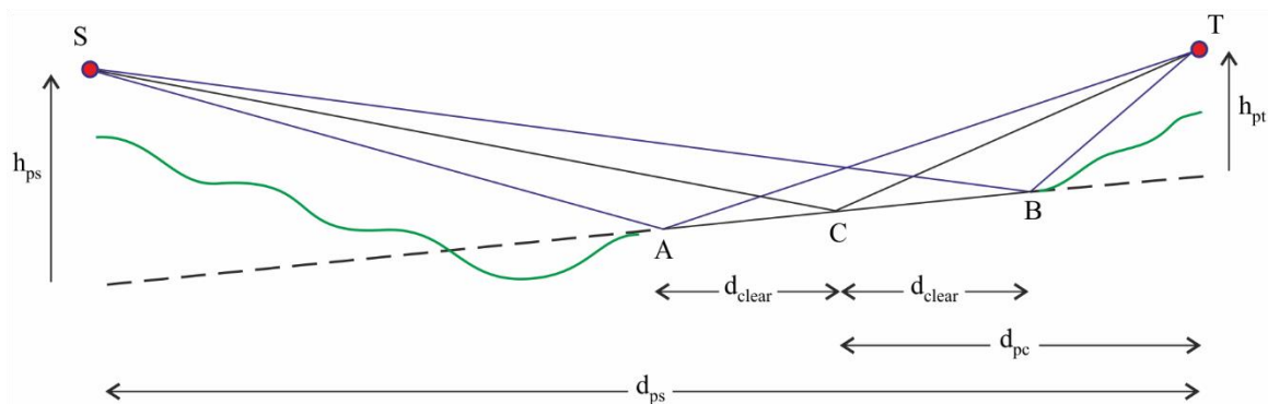
FIGURE 3 Required geometry for ground reflections
